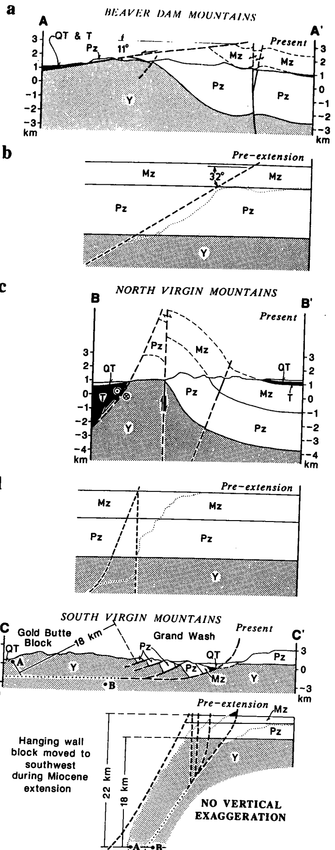
Figure 2. Balanced and reconstructed cross sections through Beaver Dam and Virgin mountains. See Figure 1 for locations and legend. B-B' and C-C' modified from Moore (1972) and Longwell (1945), respectively.
