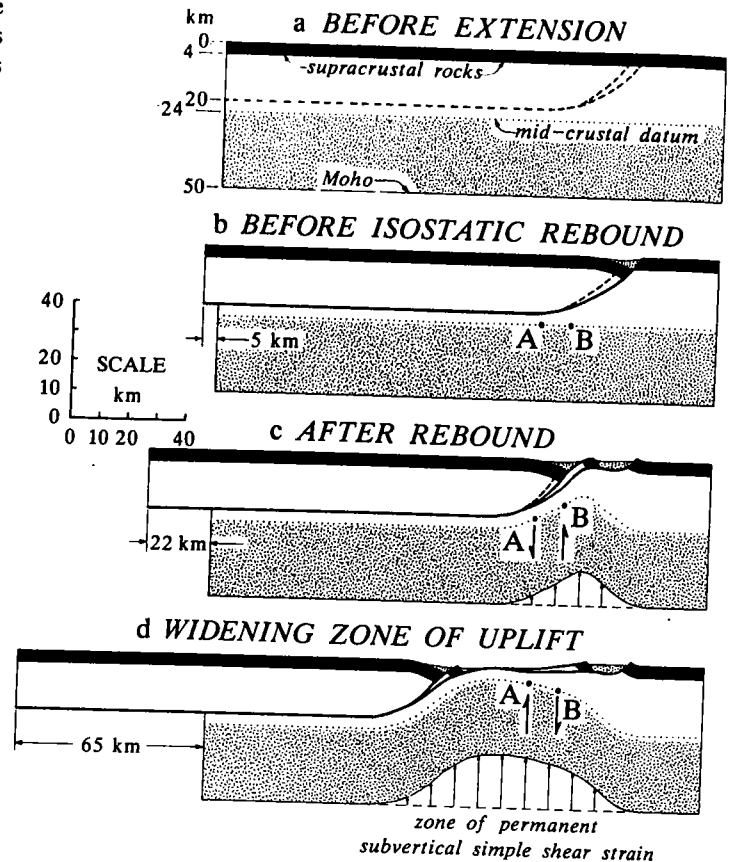
Figure 4. Conceptual model of evolving breakaway zone. Note migration of footwall strain and reversal of shear sense between points A and B.
