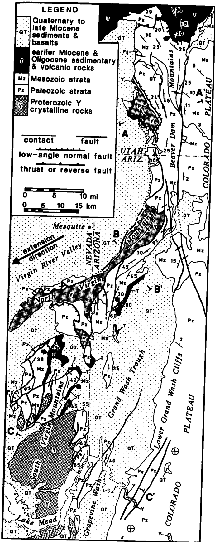
Figure 1. Geologic map of Virgin-Beaver Dam breakaway zone showing locations of cross sections in Figure 2 and critical sub-Tertiary unconformities (arrows). Compiled from Wilson et al. (1959), Volborth (1962), Beal (1965), Longwell et al. (1965), Morgan (1968), Seager (1970), Moore (1972), and Hintze (1986).
