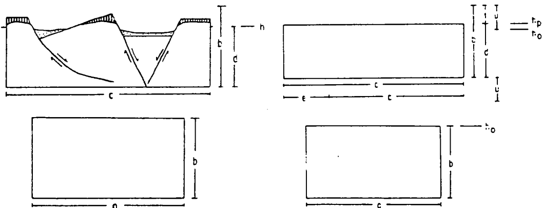
Figure 1-12. Diagram illustrating average elevation ( h ) in relation to basin-range structure. Vertically lined pattern, eroded areas; dotted pattern, depositional areas. Further explanation in text.
