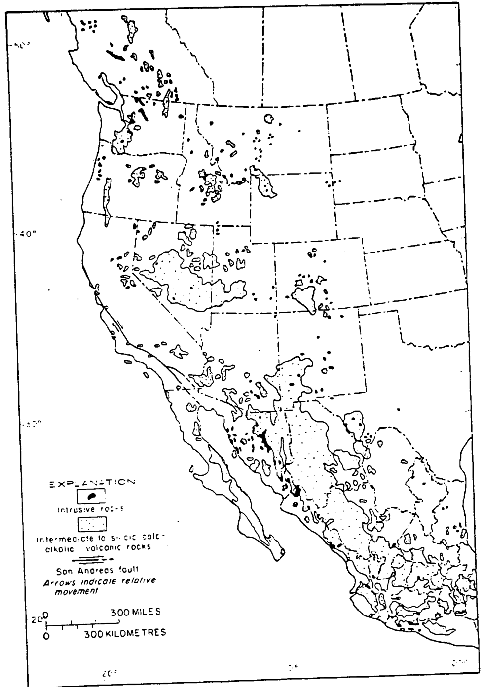
Figure 1-5. Early and middle Cenozoic (65 to 17 m.y.) igneous rocks in western North America. Compiled from Canada Geological Survey (1970b), King and Beikman (1974), Stewart and Carlson (this volume), Comite de la Carta Geologica de Mexico (1968), and Gastil and others (1975).
