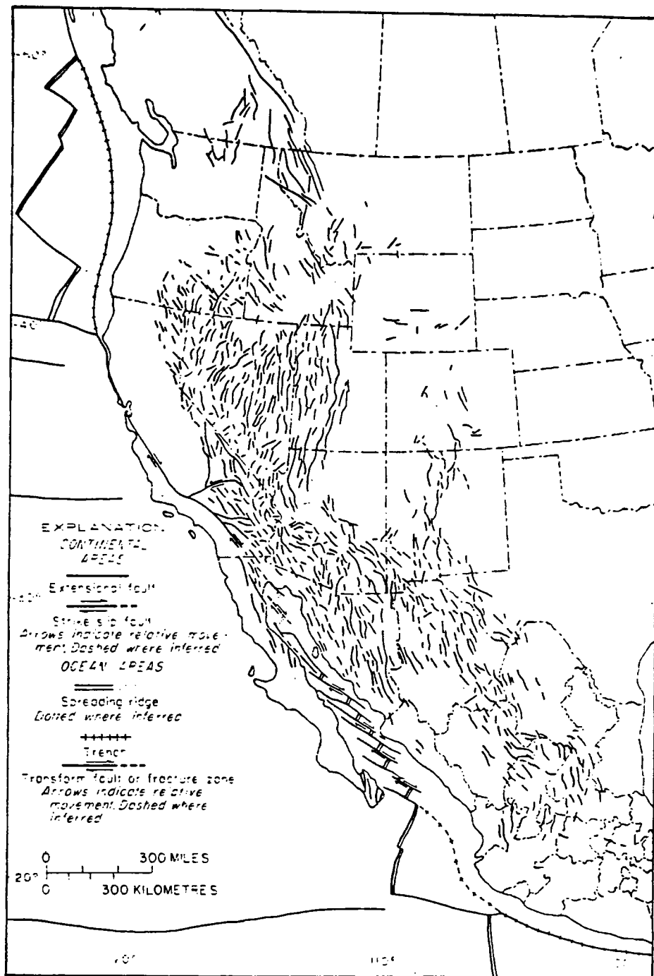
Figure 1-1. Distribution of late Cenozoic extensional faults and a few major strike-slip faults in western North America and present-day lithospheric plate boundaries. Faults are generalized and, in part, inferred. Based on various sources, including King (1969b).
