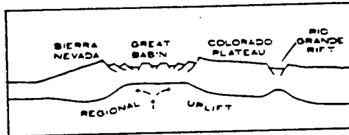
Figure 1-14. Schematic diagram illustrating regional uplift in western North America.
