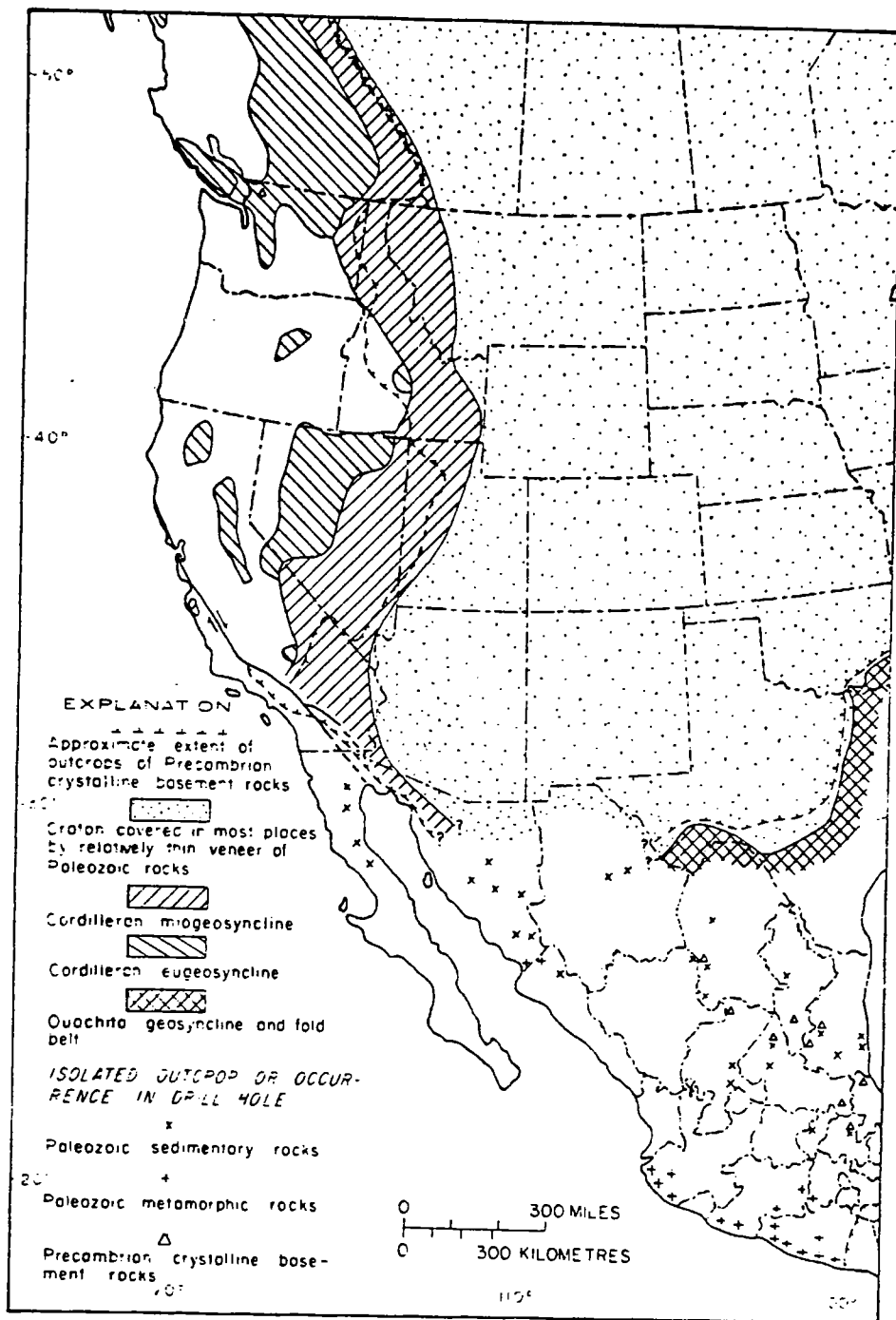
Figure 1-3. Pre-Mesozoic tectonic setting of western North America. Based on many sources, including Canada Geological Survey (1970b), Comité de la Carta Geologica de Mexico (1968), López-Ramos (1969), King and Beikman (1974), Gastil and others (1975), and Nicholas and Rozendal (1975).
