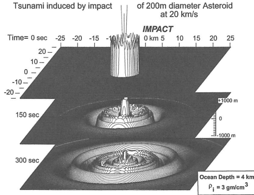
Fig. 1. Impact tsunami calculated from Eq. (2) in a uniform depth ocean (4000 m). Note that impact tsunami involve a great sequence of waves—low frequency, long waves travel fastest, shorter waves trail. The leading wave in the bottom panel is about 325m high.
