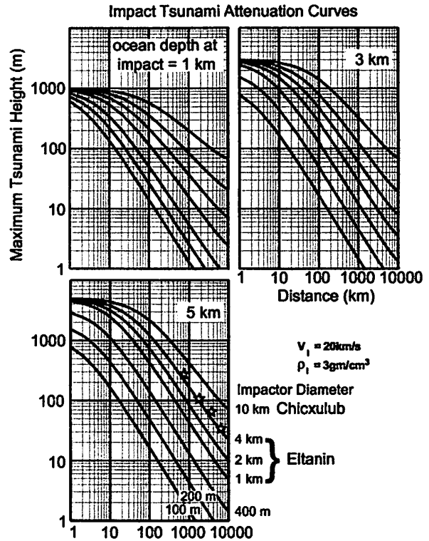
Fig. 4. Peak tsunami height computed from formula (12) versus distance and impactor diameter in oceans of h(r_0) = 1, 3 and 5 \text{ km} depth. The stars in Panel 3 mark peak tsunami amplitudes read from Fig. 3 at positions where ocean depth h(r) \approx h(r_0) . These curves do not include shoaling amplification factor (5). Green’s law [h(r_0)/h(r)]^{1/4} provides a quick approximation to this factor.
