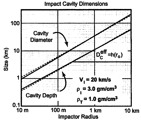
Fig. 2. Plot of initial cavity diameter d_c(R_I) and depth D_c(R_I) versus impactor radius. The solid lines come from Eqs. (7)–(9). The dashed lines come from approximations (10) and (11). For tsunami calculations, we use an effective cavity depth D_c^{eff} . D_c^{eff} equals the actual cavity depth, if D_c(R_I) does not exceed the ocean depth at impact site r_0 , otherwise D_c^{eff} = h(r_0) .
