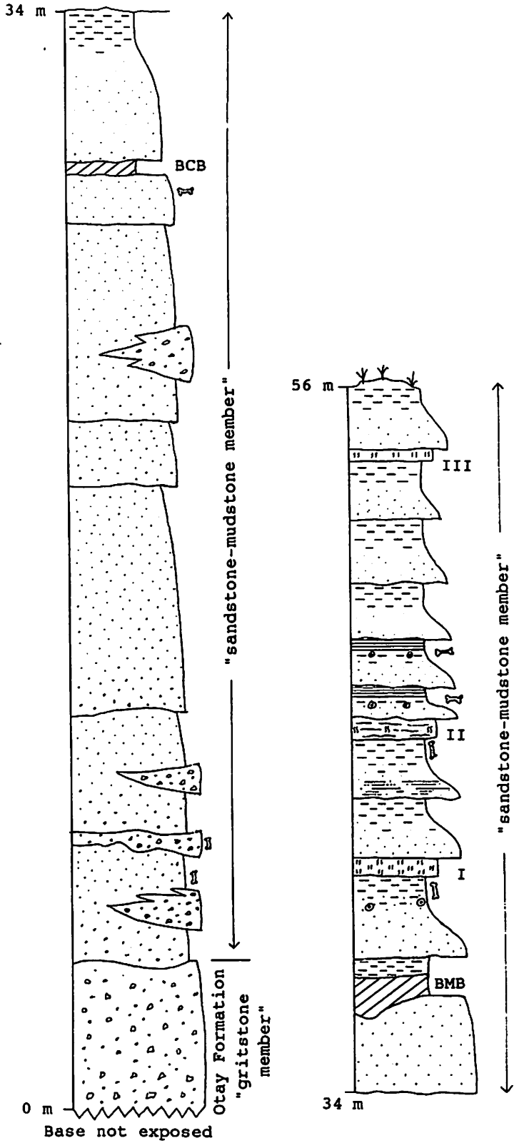
Figure 9. Measured Section 4, Eastlake Greens. Composite section measured in the Eastlake Greens development west of Lower Otay Reservoir (see Fig. 1). Possible ash beds indicated by "I", "II", and "III". BMB = "Brown Marker Bentonite"; BCB = "Business Center Bentonite."
