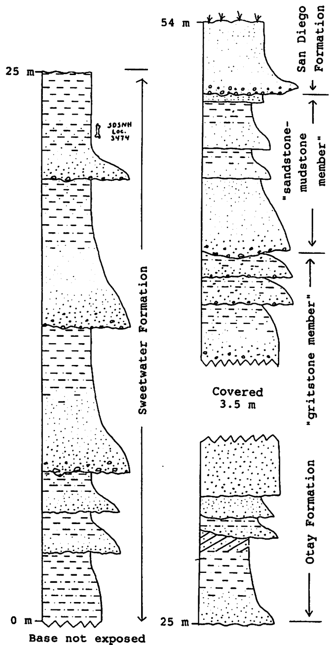
Figure 6. Measured Section 2, Bonita Long Canyon. Composite section measured in the first northwest-draining canyon north of Long Canyon (see Fig. 1).
