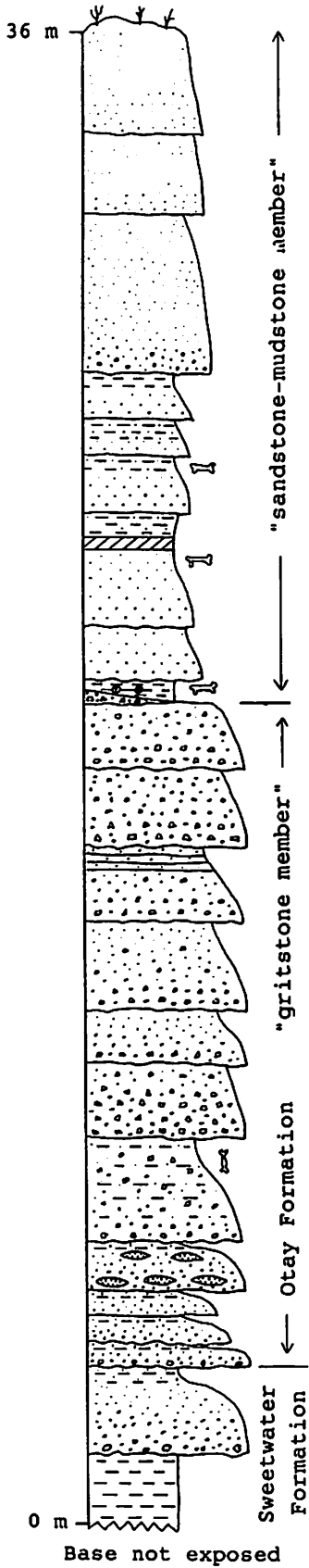
Figure 8. Measured Section 3, Salt Creek. Section measured in the Salt Creek development, Proctor Valley (see Fig. 1).
