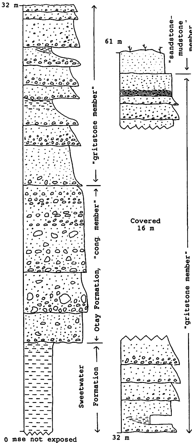
Figure 5. Measured Section 1, "Cerutti Canyon." Section measured in the second south-draining canyon east of Rock Mountain (see Fig. 1).
