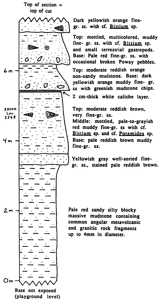
Figure 11. Measured Section 5, Mount Miguel High School. Possible intergradational contact between Mission Valley and Sweetwater formations suggested by the association of brackish-water molluscs with pale red massive mudstones. Section located at the southwesternmost corner of the Mount Miguel High School baseball fields (see Fig. 1).
