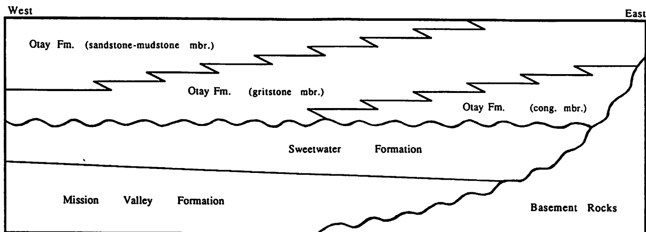
Figure 12. Proposed stratigraphic relationships of the Mission Valley, Sweetwater, and Otay formations in southwestern San Diego County.
