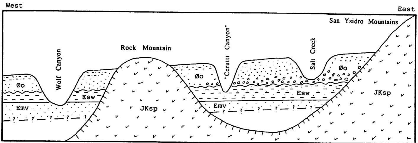
Figure 3. Generalized east-west cross-section along the north side of Otay Valley, from Wolf Canyon to the western base of the San Ysidro Mountains, showing superpositional relationships of the various lithostratigraphic units discussed in the text. Abbreviations: JKsp = Santiago Peak Volcanics, Emv = Mission Valley Formation, Esw = Sweetwater Formation, Øo = Otay Formation. Not to scale.
