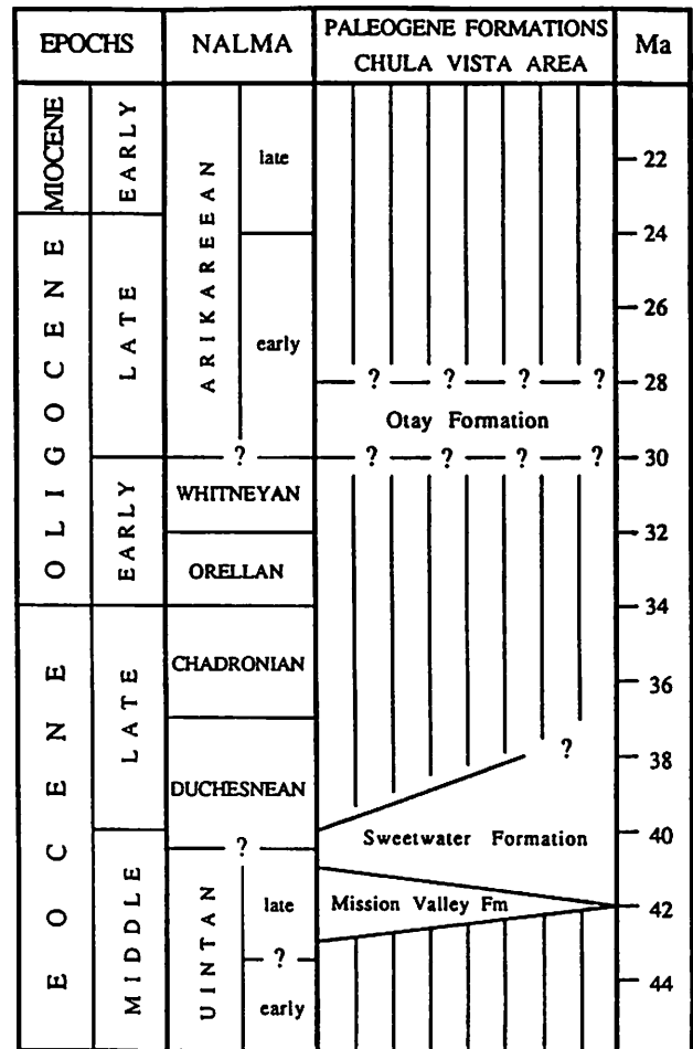
Figure 10. Age correlations for the Mission Valley, Sweetwater, and Otay formations. NALMA = North American Land Mammal "Age". Geochronometric ages of epoch and land-mammal "age" boundaries from Prothero and Swisher (1991).
