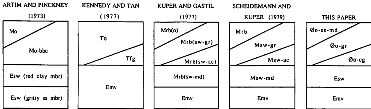
Figure 2. Summary of the history of stratigraphic nomenclature for the Sweetwater and Otay formations in southwestern San Diego County. Abbreviations: T = Tertiary, E = Eocene, Ø = Oligocene, M = Miocene, ac = angular conglomerate facies, bbc = basal breccia conglomerate unit, cg = conglomerate member, fg = fanglomerate unit, gr = gritstone member or facies, md = mudstone facies, mv = Mission Valley Formation, o = Otay Member or Formation, rb = Rosarito Beach Formation, ss-md = sandstone-mudstone member sw = Sweetwater Member or Formation.
