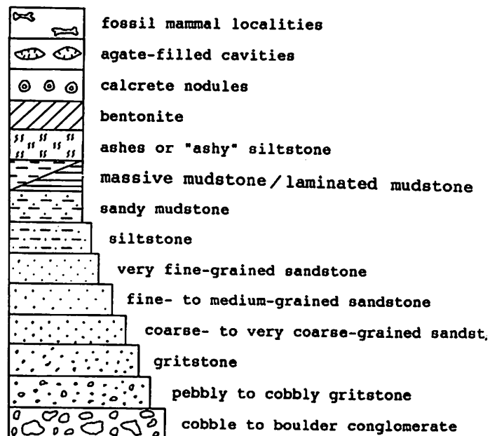
Figure 4. Key to lithologic symbols used in Measured Sections 1-5.
