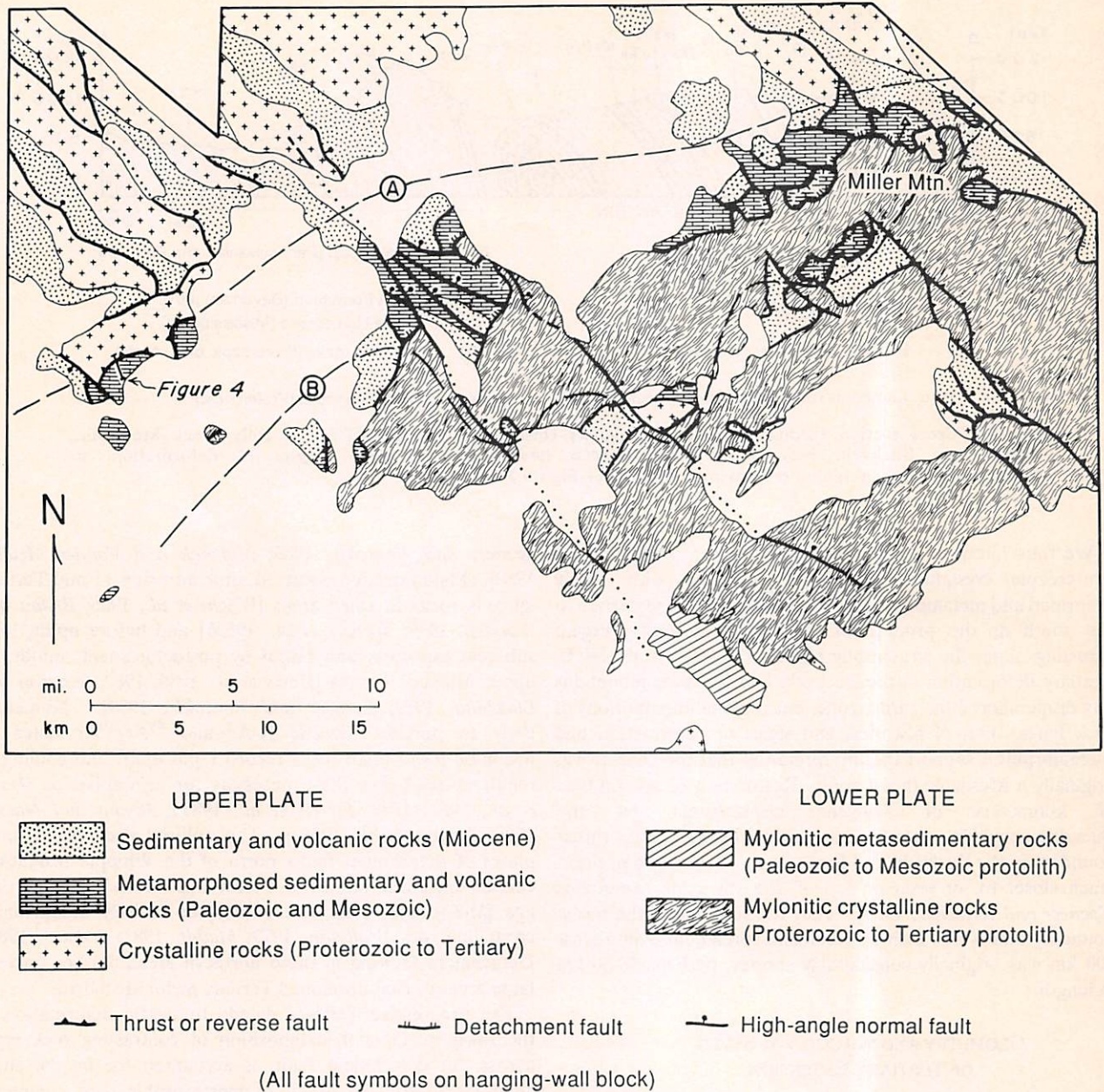
Fig. 3. Simplified geologic map of upper and lower plate rocks in the Buckskin and Rawhide Mountains and adjacent areas (modified from Spencer [1989]). Dashed line A represents dismembered, discontinuously exposed, structurally highest thrust of MFTB. Dashed line B represents approximate southward termination of pre-Tertiary upper plate rocks; primarily Tertiary rocks rest on detachment fault south of this line.
