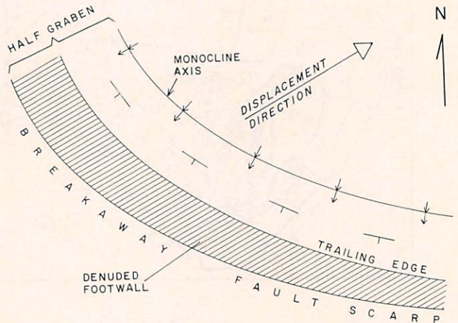
Fig. 6. Schematic diagram of structural relationships along an oblique breakaway zone. Illustrated case is for listric fault with the same curvature for all cross sections perpendicular to the top of the breakaway fault scarp. Modified from Figure 16 of Dokka [1986].
