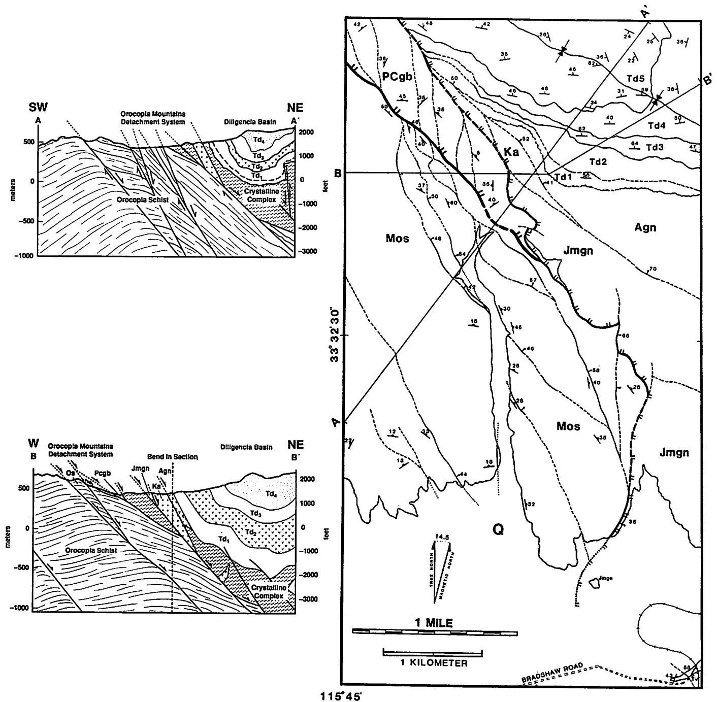
Figure 2. A geologic map of a portion of the Orocopia Mountains. The thick line represents the contact between upper and lower plate along the Eocene mylonitic boundary called the Orocopia Mountains Detachment Fault (OMDF), double ticks are on the hanging wall. The thinner double ticked line is the Diligencia Detachment Fault (DDF) which is shown to truncate OMDF in the central portion of the map. Map units are designated: Lower plate; Mos, is the Mesozoic Orocopla Schist. Upper plate; PCgb, is a blue quartz banded gneiss of possible Precambrian age; Jmgn, is a suite of mafic gneiss including diorite, gabbro and anorthosite; Agn, is an alkali feldspar augen gneiss; Ka, is a tabular unit of adamellite. Diligencia basin sedimentary rocks; Td1 through Td5 are part of the early Miocene Diligencia Formation with Td3 being the 20-23 Ma basalt; Tv represents volcanic rocks in the southeastern map area that are tilted back into DDF as it trends south out of the range. Q, is Quaternary alluvium. Figure 2A is a cross section from A-A' and Figure 2B is a cross section from B-B' across the Orocopia Mountains Detachment System.
