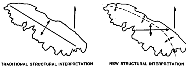
Figure 5. The traditional structural representation of the Orocochia Schist package as a northwest-oriented antiform and a new interpretation based on TM imagery and aerial reconnaissance which depicts an east-plunging antiform with a smaller scale antiformal rollover developed below the upper-plate/lower-plate contact.
