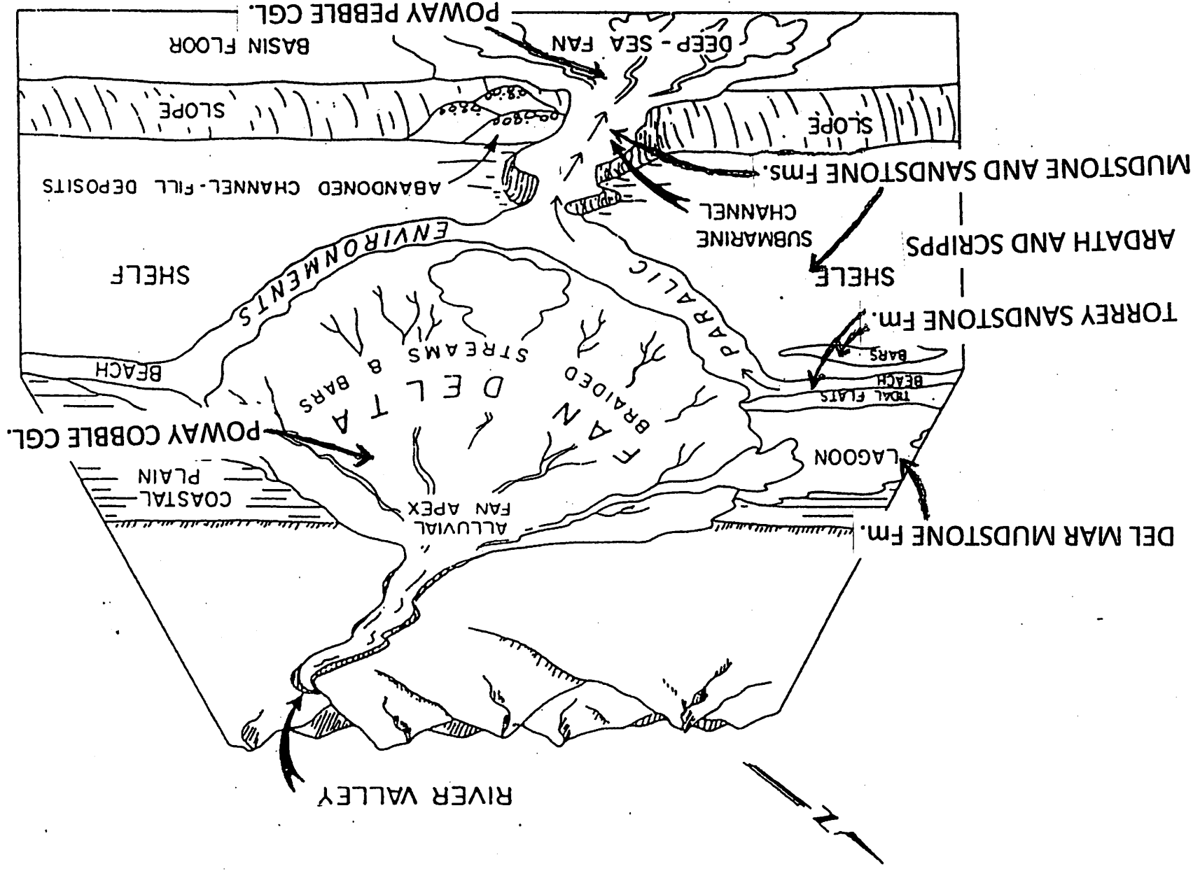
Figure 1. Depositional model for middle and upper Eocene strata in the San Diego area. From Link et al., 1979.
