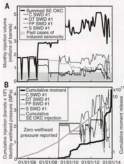
Fig. 3. Fluid injection reported in the four high-rate SE OKC wells. (A) Sum and individual monthly injection volumes and (B) wellhead pressure and cumulative, summed injected volume (15). The DT SWD #1, FP SWD #1, and S SWD #1 wells are in close proximity; the C SWD #1 well is \sim 3.5 km away. Gray shading denotes injection rates for notable past cases of induced seismicity for reference (table S1). Cumulative seismic moment in (B) is calculated from M3+ earthquakes from 2005 to January 2014 (10) for earthquakes within the box outlining the Jones swarm in Fig. 1.
