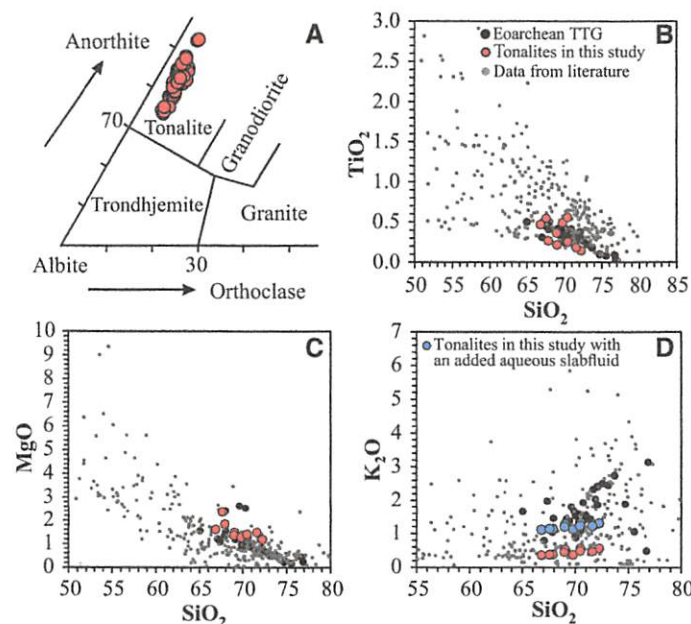
Figure 1. A: Normative anorthite-albite-orthoclase classification diagram showing that melts in this study are tonalitic in composition. B–D: Representative TiO_2 - SiO_2 , MgO - SiO_2 , and K_2O - SiO_2 variation diagrams. TiO_2 - SiO_2 and MgO - SiO_2 data illustrate similar liquid lines of descent of our tonalites with regards to published Eoarchean tonalite, trondjemite, and granodiorite (TTG) data (Hoffmann et al., 2011; Nutman et al., 2009). Previous experimental liquids (see data in Table DR4 [see footnote 1]) can overlap Eoarchean TTG data, but are, for most part, highly variable. K_2O - SiO_2 plot shows that our data can only intersect Eoarchean data if aqueous slab-derived fluid is involved.
