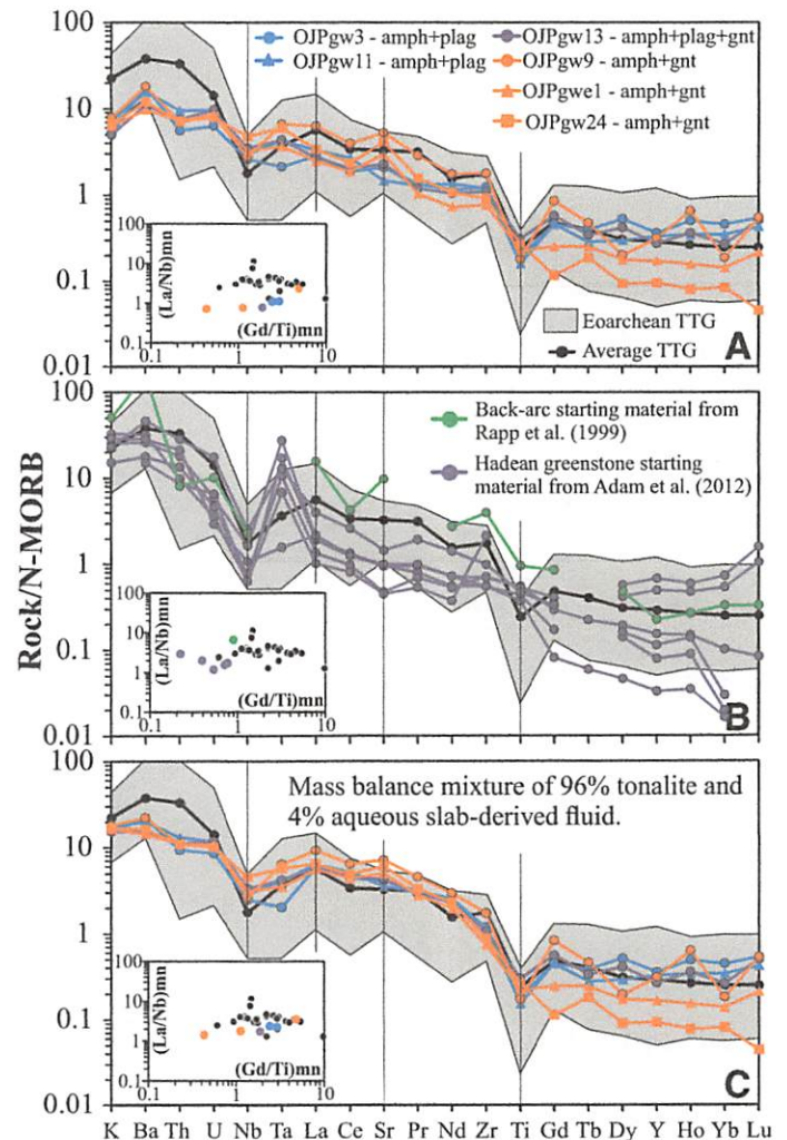
Figure 2. A: Normal mid-oceanic ridge basalt (N-MORB)-normalized multi-element diagram showing trace element contents of our experimentally derived melts relative to Eoarchean tonalite, trondjemite, and granodiorite (TTG) (Hoffmann et al., 2011; Nutman et al., 2009). Key shows residual aluminum-bearing phase(s) in equilibrium with melt (amph—amphibolite; gnt—garnet; plag—plagioclase). B: Multi-element diagram showing trace element contents of experimental liquids derived from Hadean greenstone and back-arc starting materials (Adam et al., 2012; Rapp et al., 1999). C: Multi-element diagram showing trace element contents of our tonalites that have been mixed with slab-derived aqueous fluid. All diagrams have inset MORB-normalized (mn) La/Nb - Gd/Ti plot to illustrate magnitude of negative Nb and Ti anomalies discussed in text.
