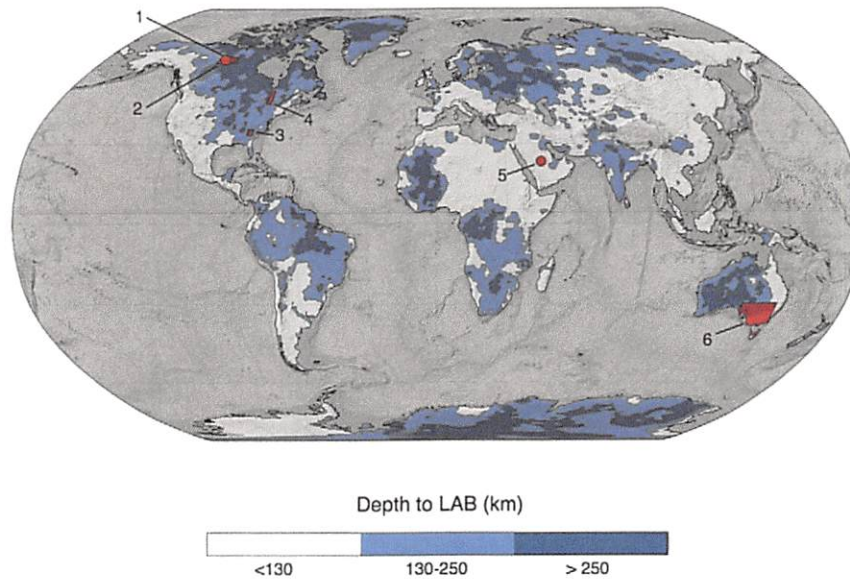
Fig. 5. Contours of continental lithosphere thickness taken from the litho1.0 model (Pasyanos et al., 2014). Dark blue are the regions thicker than 250 km and lighter blue are regions between 130 and 250 km in thickness. Thinner regions have not been colored. The background is shaded relief computed for ETOPO1 (Eakins and Amante, 2009). Red polygons indicate the locations of broadband seismic studies that observe structures that have been interpreted to be ancient accreted terranes/terrane boundaries preserved within the continental lithosphere (1 – Bostock, 1998; 2 – Cook et al., 1998; 3 – Parker et al., 2015; 4 – Rondenay et al., 2000; 5 – Levin and Park, 2000; 6 – Pilia et al., 2015).
