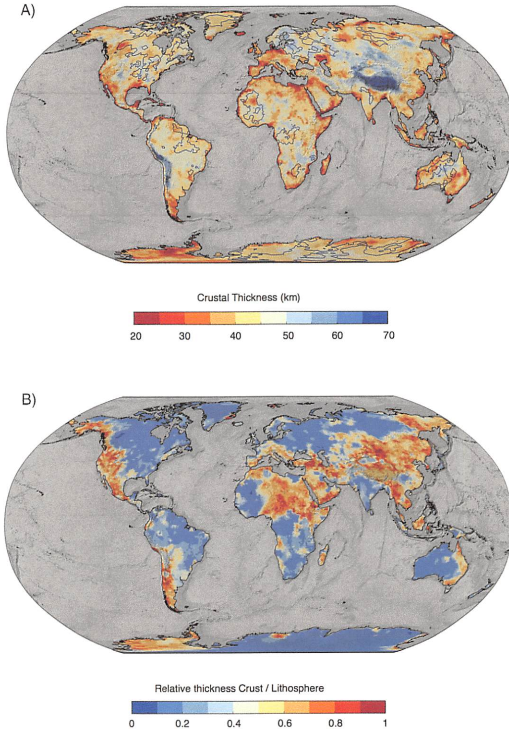
Fig. 2. The thickness of the continental crust (A) and the relative thickness of the continental crust to total lithospheric thickness (B) both derived from the layer thickness maps of litho1.0 (Pasyanos et al., 2014). In A, we have outlined those regions where the depth to the lithosphere-asthenosphere boundary is >250 km.
