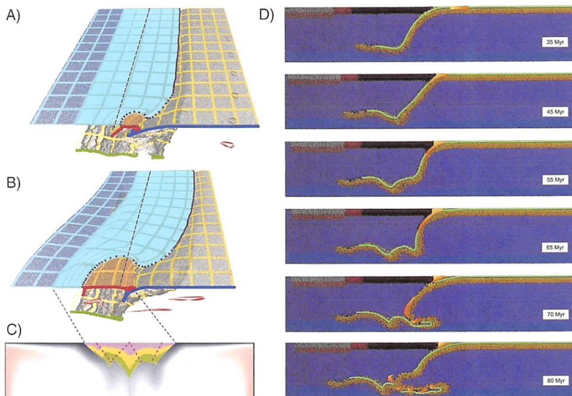
Fig. 8. Three dimensional models of accretion of (A) a 250 km and (B) a 500 km radius oceanic plateau (shown with orange markers) into a deformable margin (snapshots of movies from Moresi and Willis (2015) showing only their marker surfaces). The oceanic plate is grey with a yellow strain-marker grid. The continental crust is dark blue with a light grid. Transitional crust is cyan with a grey grid. The indenting plateau is orange. The plate boundary is a purple dotted line. The dark, dashed line indicates the position of the trench at the onset of collision. The colored lines indicate the cross-sectional view of the pre-collision lower-plate lithosphere (green), the plateau (red), and the post-collision lower-plate lithosphere (blue). (C) shows the correspondence between the high-resolution 2D, thermal-mechanical models of Cooper and Miller (2014) and the compositional-mechanical 3D models. (D) is a cross section through the collision of a 125 km radius plateau showing all material elements (Betts et al., 2015) and illustrating a geometry similar to that of the Yakutat subduction and accretion.
