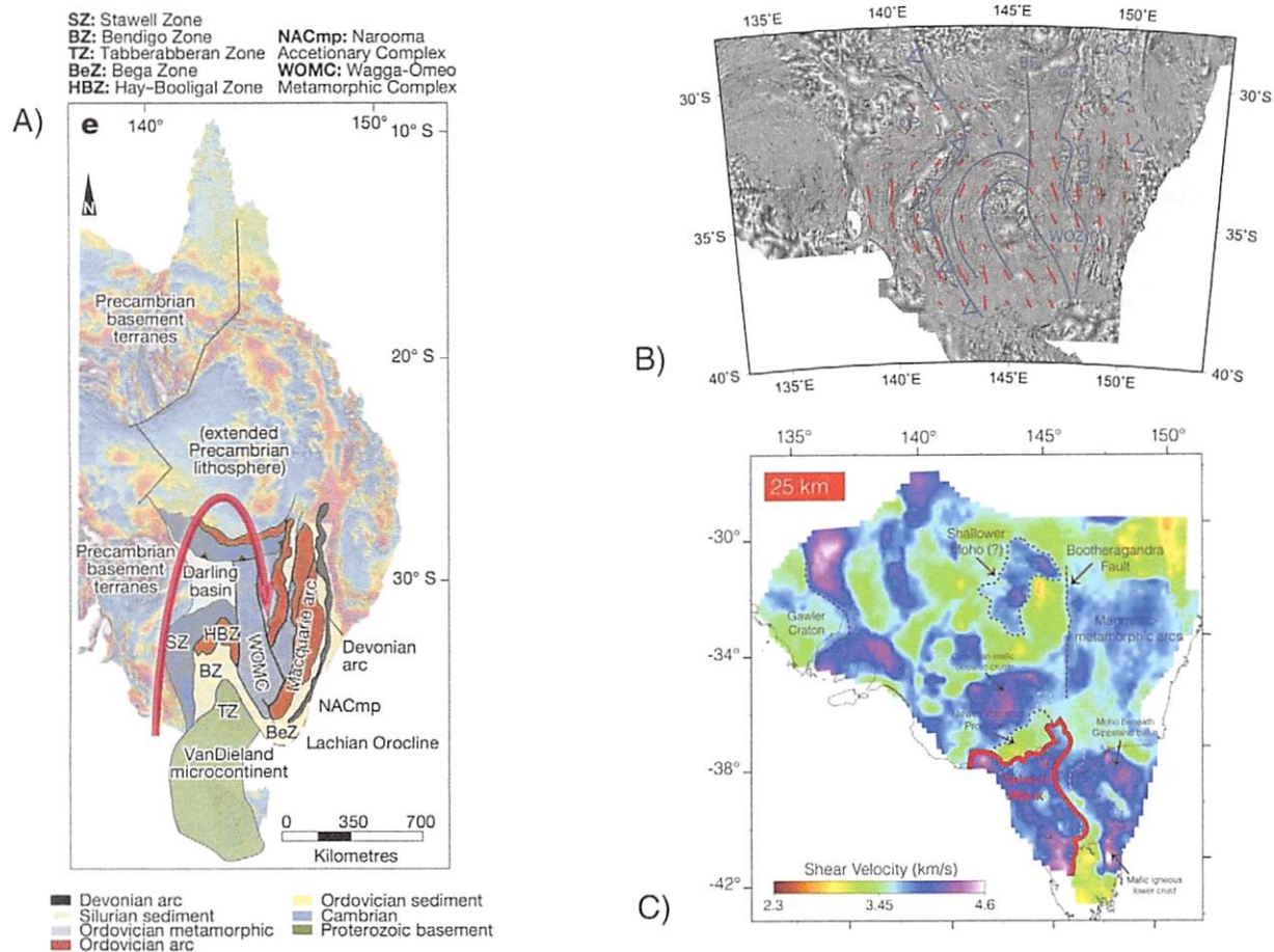
Fig. 9. (A) is a simplified regional tectonic map of the southern and central Tasmanides superimposed on a magnetic intensity map of eastern Australia (figure from Moresi et al., 2014). The curved red arrow shows the sense of overall motion predicted by numerical models and inferred from the geological and geophysical interpretation of Cayley (2011). (B) the orientation of the seismic fast direction (dark red vectors) superimposed on magnetic data with an interpretation of the inferred fabric shown in blue (figure from Rawlinson et al., 2014). (C) Seismic shear-wave velocity anomalies at 25 km from the regional tomographic model of Piliá et al. (2015) with their outline of the seismic signature of the Selwyn block at depth (red contour).
