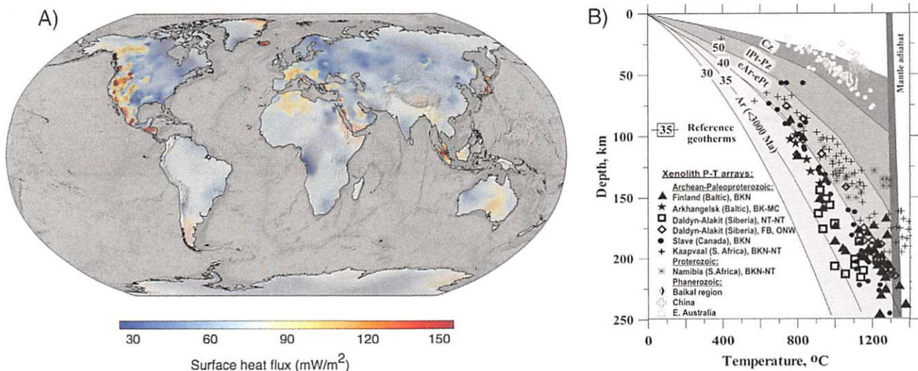
Fig. 3. (A) Global surface heat flow measurements (International Heat Flow Commission) plotted by binning the point-measurement datasets to an adaptively-refined triangulation with a minimum resolution of 50 km. Color saturation represents the resolution of the triangulation which washes out progressively such that the coarsest resolution is shown with only 5% saturation. (B) Lithospheric geotherms for continental regions (figure from Artemieva, 2009).
