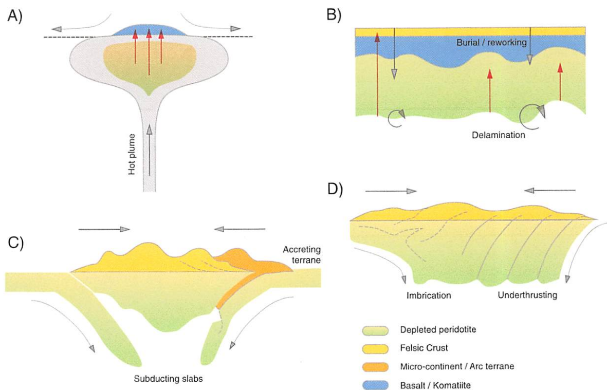
Fig. 7. Conceptual sketches of craton formation. Grey arrows show sense of motion. Red arrows indicate melt transport. (A) Melting event triggered by large mantle plume as described in Pearson et al. (1995) and Lee et al. (2011). (B) Burial/reworking and sorting of dense materials (e.g., Robin and Bailey, 2009; Moore and Webb, 2013; Sizova et al., 2015). Though not explicitly shown in this sketch, diapirism can further aid the resorting of dense materials. (C) Lithospheric thickening through the amalgamation of arc material (e.g., Jordan, 1978). (D) Thrust stacking and imbrication of buoyant oceanic lithosphere (e.g., Bostock, 1998).
