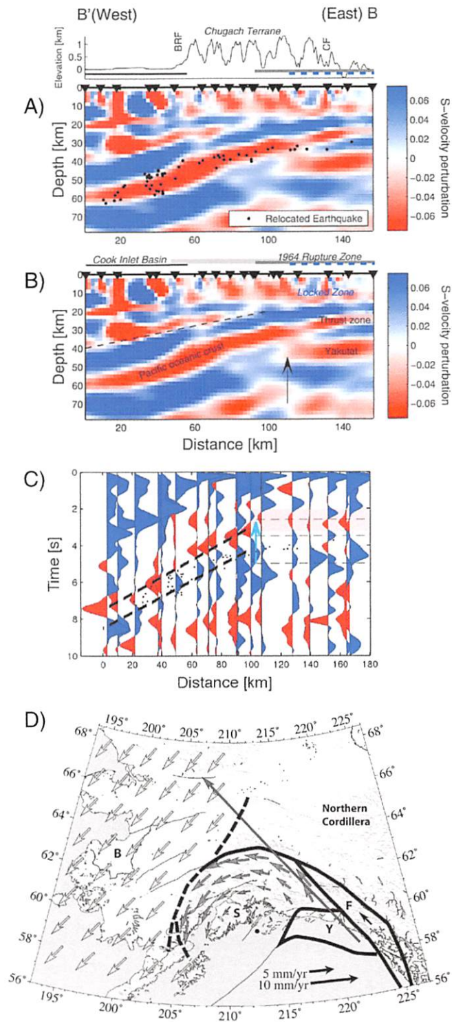
Fig. 10. (A-C) Seismic discontinuity imaging from (Abers et al., 2014) in southern Alaska showing a profile (B-B') that cuts obliquely across the subducting portion of the Yakutat terrane. The interpreted seismic images show the low-velocity Pacific oceanic crust and the westernmost extent of the Yakutat terrane being subducted beneath the Chugach terrane on the North American plate. The arrows indicate the position of the Yakutat in both the GRT based images (see Abers et al. (2014) for details) and the stacked P receiver functions. (D) Freymueller et al. (2008) block rotation model for the Alaskan syntaxis showing the Yakutat block indenter and the escape of material westward and southward. (E) shows a simplified tectonic map of Alaska (Colpron et al., 2007) that highlights the long history of accretion, the present day orocline, and the dissection of the margin by the incoming Yakutat block. The yellow patch indicates the approximate extent of the subducted Yakutat crust from (Eberhart-Phillips et al., 2006) and the red line is the location of the profile (B-B') in the left hand column (A-C). (Eberhart-Phillips et al., 2006).
