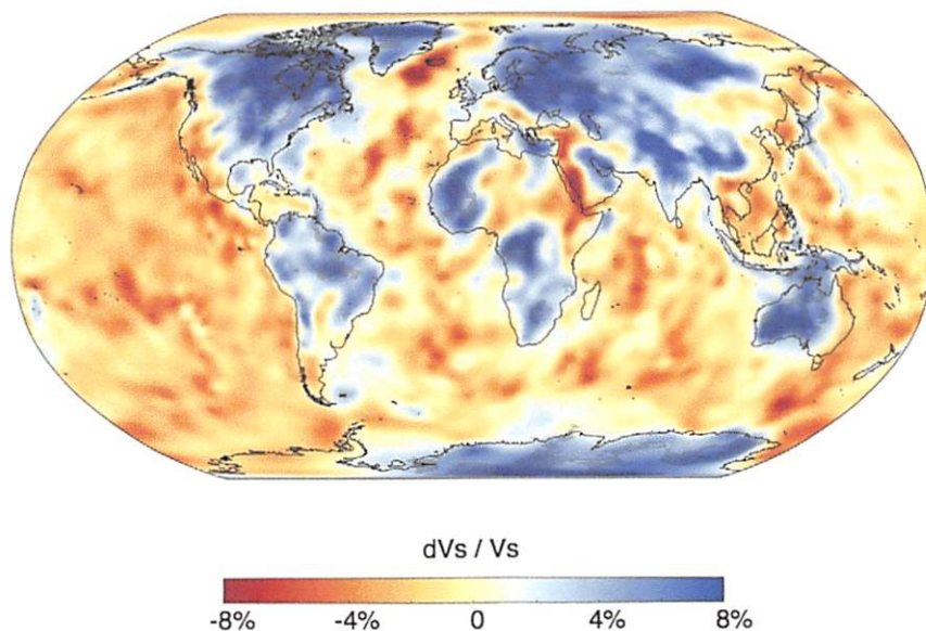
Fig. 4. Global S wave tomography model by Schaeffer and Lebedev (2013) plotted at 150 km depth. The additional shading indicates regions with very thick (>250 km) lithosphere in the litho1.0 model (Pasyanos et al., 2014).
