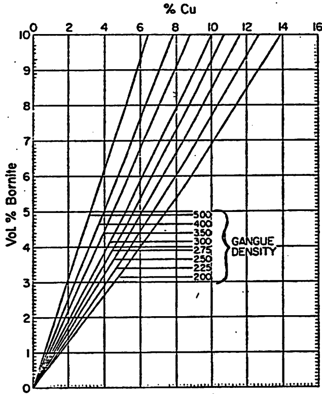
Volume percent Bornite to weight percent copper, For variable gangue density. Calculated assuming bornite is 63.3% copper with a density of 5.07. For rough visual estimates, volume % bn ≈ weight % cu, for gangue densities of about 3.
