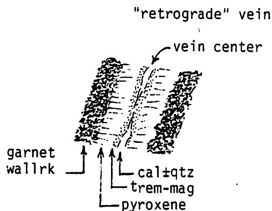
Figure 5. Vein mineralogy.
