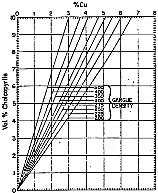
Volume percent chalcopyrite to weight percent copper, For variable gangue density. Calculated assuming chalcopyrite is 34.64% copper with a density of 4.28. For rough visual estimates, 1/2 volume % cp ≈ weight % cu, for gangue densities of about 3.
