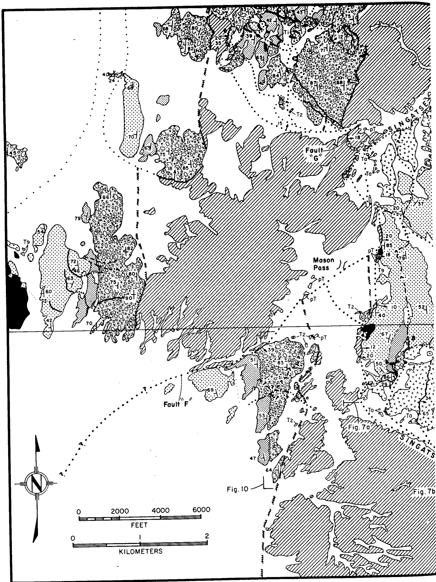
Figure 5. Generalized geologic map of part of Yerington district, Nevada.
