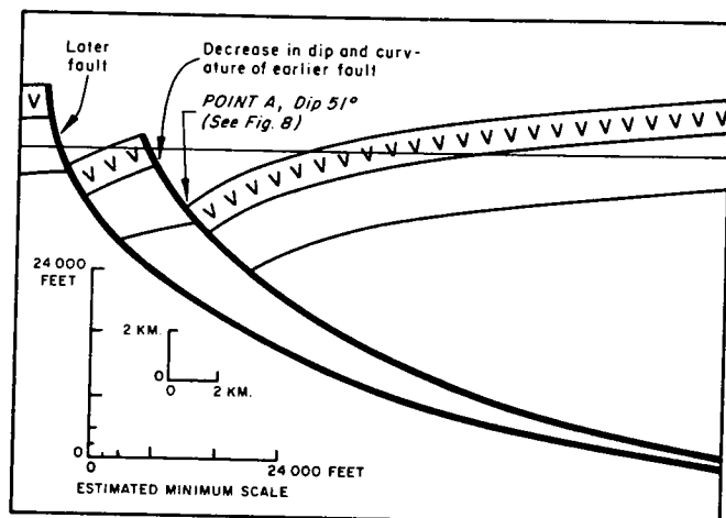
Figure 13. Tilting and reduction of dip and curvature of early normal fault (fault of Fig. 8) by tilting due to displacement on later normal fault. Note that vertical displacement as well as tilting are due to hanging-wall block adjusting in shape to fill a potential void resulting from horizontal extension between hanging wall and footwall. Hanging wall could have adjusted to its new shape by development of antithetic faults instead of tilting, as has clearly been shown by Hamblin (1965), but in Yerington district tilting was dominant.
