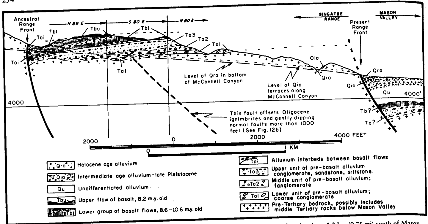
Figure 6. East-west cross section showing 8- to 11-m.y.-old basalt and alluvium and Quaternary deposits about 1.2 km (0.75 mi) south of Mason.
