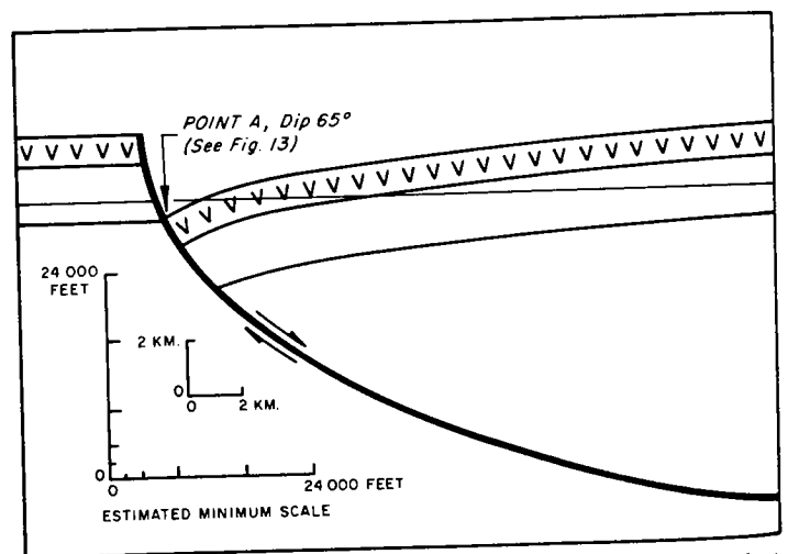
Figure 8. Cross section showing idealized fault of type found at Yerington, showing decrease in dip, inferred decrease in concave-upward curvature with increasing depth, and increase in tilting of hanging-wall rocks toward fault. Scale is estimated from available data as discussed in text, but depth shown at which fault becomes flat is probably a minimum.
