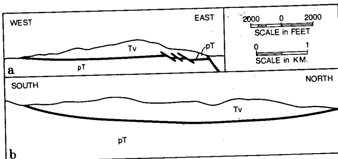
Figure 7. East-west section (a) and north-south section (b) across Singatse fault (see Fig. 5), showing Tertiary volcanic rocks (TV) and pre-Tertiary rocks (pT).
