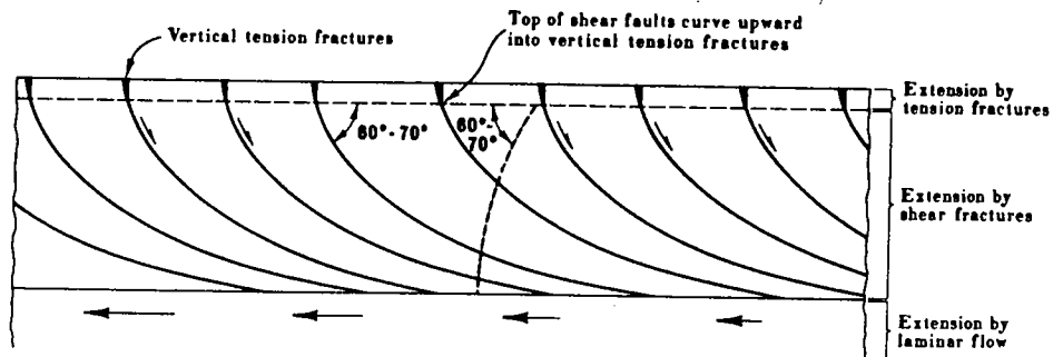
Figure 16. Possible mechanical model for Basin and Range faulting in Yerington district, shown on east-west cross section looking north. Depth of suggested change from tension to shear failure is not determined, but observational data suggest it is not deep. Walls of upper tension-fracture part of structure probably collapse, resulting in what appears to be near-vertical normal or reverse fault (as westernmost fault in Fig. 6). Deep-seated antithetic faults (dashed fault) are suppressed, perhaps because potential voids would result at base of cell. However, shallow antithetic faults could form in hanging wall of east-dipping normal faults instead of tilting (Fig. 14).
