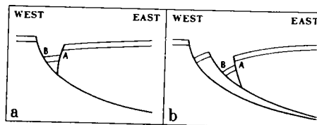
Figure 14. Diagrammatic cross section showing antithetic normal fault A at time a, changed to reverse fault at later time b due to westward tilting on east-dipping normal fault. Note that antithetic fault A developed in place of westward tilting in hanging wall block of fault B.
