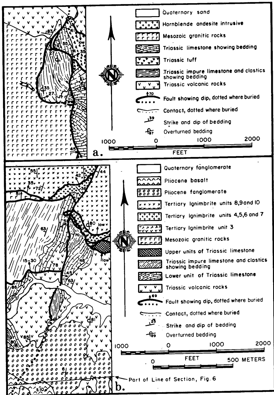
Figure 12. a, Moderately east-dipping normal fault cut by slightly steeper one. b, South flanks of gently dipping trough-shaped faults cut by moderately east-dipping fault (see Fig. 2 for locations).
