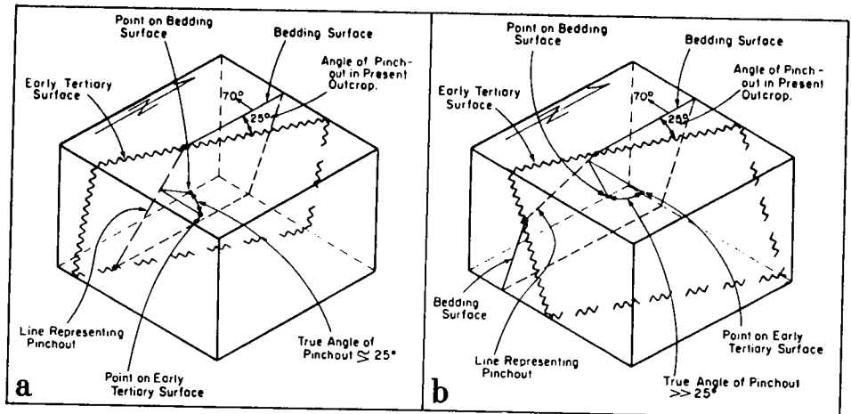
Figure 11. a, Block diagram of pinch-outs of Figure 10. Average strike of early Tertiary surface, strike and dip of bedding, and angle of pinch-out in present outcrop (about 25°) are known (variations in present topography, not shown in Fig. 10, have been taken into account). Slope of early Tertiary hill (= true angle of pinch-out) could not have been greater than about 35°, so true angle of pinch-out is equal to or slightly (as much as 10°) greater than angle of pinch-out in present outcrop. Therefore, average dip of early Tertiary surface must be such that line representing pinch-out is perpendicular to strike of bedding or diverges from perpendicular to strike by a certain limited angle. If true angle of pinch-out was as high as 35° (not likely), then variance of line of pinch-out from perpendicular to strike could have been as much as 60° if pinch-out line plunged north or 40° if it plunged south. Even such an unlikely high variance from perpendicular-to-strike results in a small error in calculating direction of displacement (Fig. 11c). b, If line representing pinch-out was nearly parallel to strike of bedding, as in example illustrated, then slope of early Tertiary hill (= true angle of pinch-out) would have to be unreasonably high. c, Diagram shows that for gently dipping faults, error in calculating net displacement direction from an offset pinch-out line is much smaller than error in estimating orientation of line of pinch-out. Average overall dip of Singatse fault is only about 3° (exaggerated in diagram), which would result in maximum possible error of about 5° (exaggerated) in determining displacement direction for Singatse fault.
