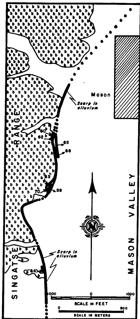
Figure 9. Outcrop map of range-front fault southwest of Mason (see Fig. 2 for location) that has been active in Holocene time. Blank area is Quaternary alluvium, "b" pattern is bed rock.
