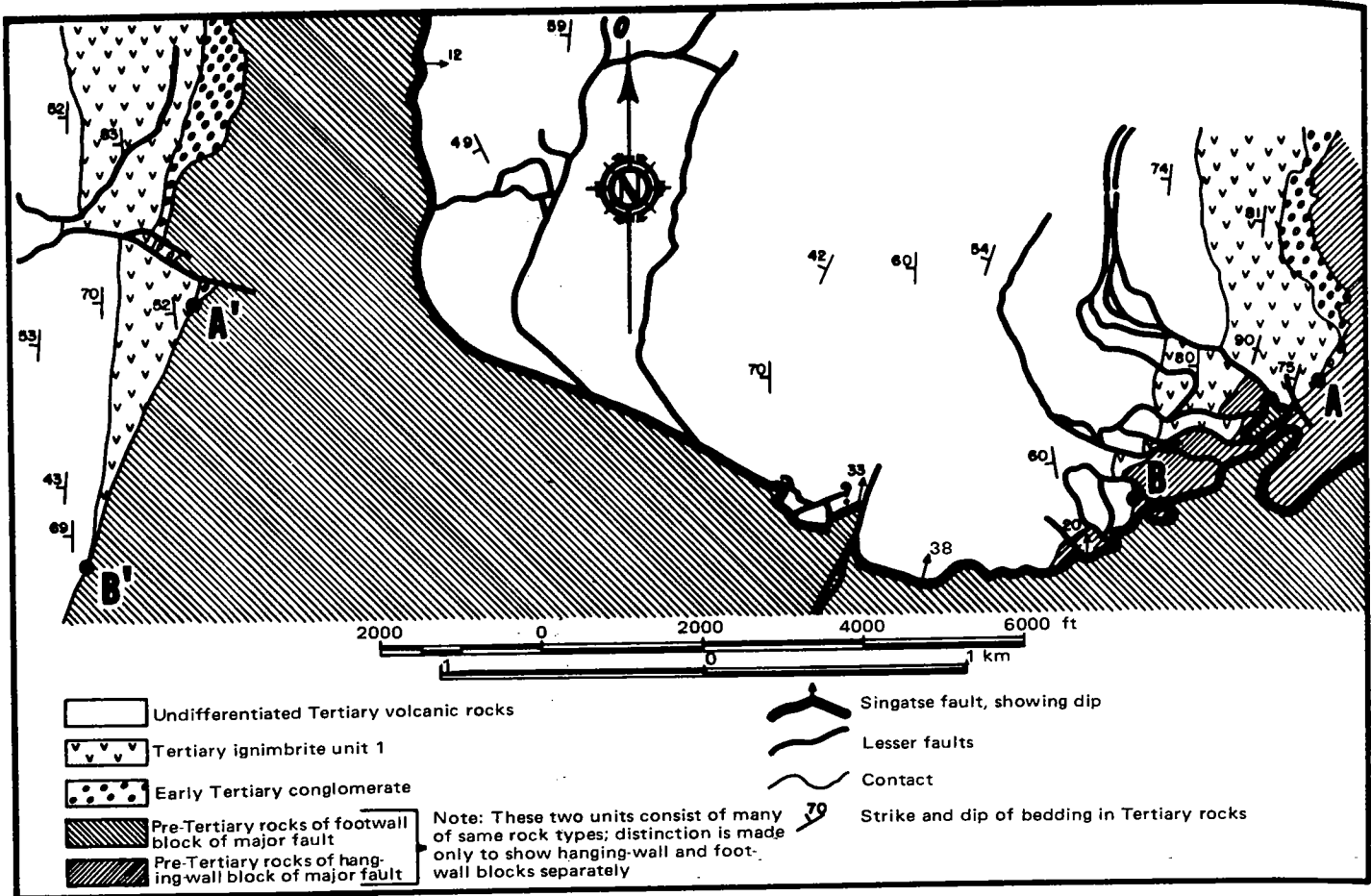
Figure 10. Singatse fault, showing offset units that pinch out in its hanging wall and footwall.
