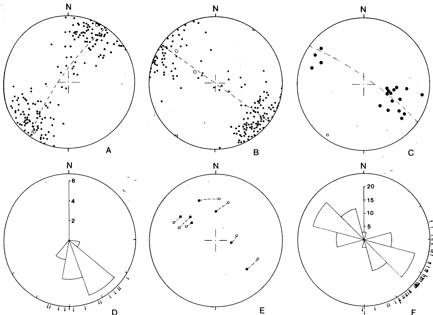
Figure 7. Structural data from the Schoonover sequence. A. Fold axes. B. Poles to axial plane. In A and B, dots are first-generation structures, and open circles represent clear-cut examples of second-generation structures. C. Poles to thrust-fault planes measured in D (dots), and pole to great circle formed by these (square). D. Rose diagram of calculated slip directions on small-scale thrust faults that cut the hinges of folds. E. Comparison of calculated slip directions (open circles) and measured striations and slickensides (dots) on seven small-scale thrust faults. F. Striations and slickensides on small-scale faults of unknown sense of offset and on bedding surfaces along basal thrust of Schoonover sequence, and along the base of higher thrust plates.
