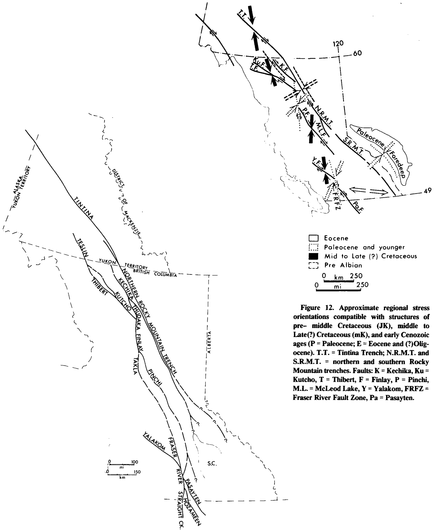
Figure 11. Regional continuation of faults in the Cordillera. S.C. = Shuswap Complex.
