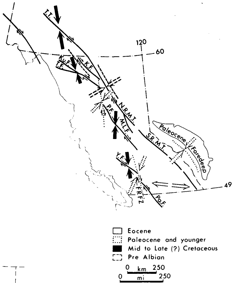
Figure 12. Approximate regional stress orientations compatible with structures of pre- middle Cretaceous (JK), middle to Late (?) Cretaceous (mK), and early Cenozoic ages (P = Paleocene; E = Eocene and (?) Oligocene). T.T. = Tintina Trench; N.R.M.T. and S.R.M.T. = northern and southern Rocky Mountain trenches. Faults: K = Kechika, Ku = Kutcho, T = Thibert, F = Finlay, P = Pinchi, M.L. = McLeod Lake, Y = Yalakom, FRFZ = Fraser River Fault Zone, Pa = Pasayten.
