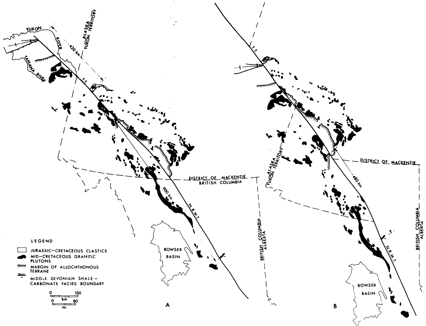
Figure 10. Reconstruction for offsets along the Tintina Trench and N.R.M.T. Data from Roddick, 1967; Tempelman-Kluit, 1977; Beikman, 1980; and Gordey, 1981. Note that the restoration of ~420 km, obtained by matching the Jurassic-Cretaceous clastics, still leaves the Middle Devonian facies boundaries 480 km apart.
