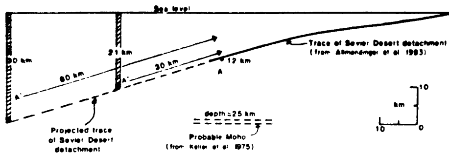
FIG. 4 Diagram showing possible initial overburden on the deepest clearly visible part of the Sevier Desert detachment.
