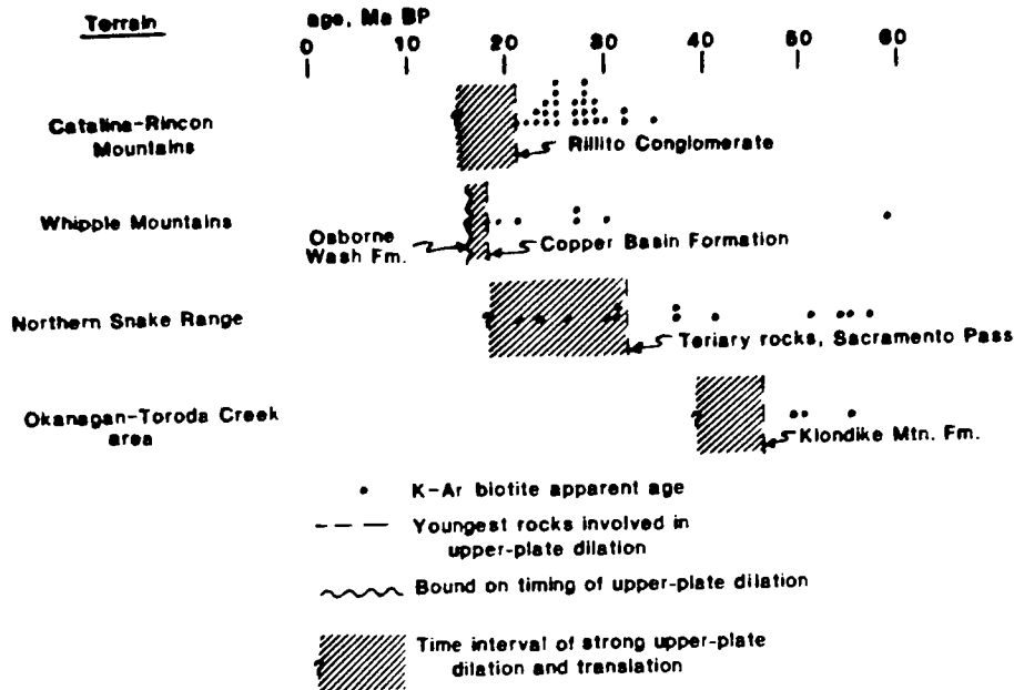
FIG. 2. Age relations between cooling of lower-plate tectonites and timing of latest upper-plate imbricate normal faulting and brittle detachment. Significant amounts of upper-plate dilation and translation probably occurred in all of these terrains prior to the deposition of the youngest rocks involved in the deformation; thus the shaded areas represent only the latest phase of significant upper-plate strain. Sources: Catalina-Rincon mountains, Keith et al. (1980) and M. Shafiqullah and H. W. Peirce (unpublished data); Whipple Mountains, Davis et al. (1982); northern Snake Range, Miller et al. (1983 and unpublished data) and Lee et al. (1980); Okanagan - Toroda Creek area, Fox et al. (1977) and Pearson and Obradovich (1977).
