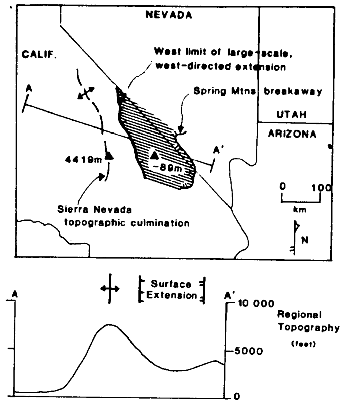
FIG. 15. Map and cross section showing breakaway, area of surface extension, position of topographic axis, and topographic profile across part of southern Nevada and central California. Triangles show locations of highest and lowest points in the coterminous United States. The zone of extensional allochthons depicted here is currently active.
