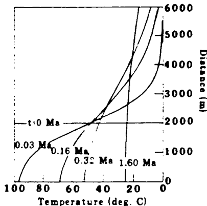
FIG. 5 Time versus temperature profile for conductive decay of a 100^{\circ}\text{C} temperature step in rocks with thermal diffusivity of 1.3 \times 10^{-7} \text{ m}^2 \text{ s}^{-1} , adapted from Carslaw and Jaeger (1959).
