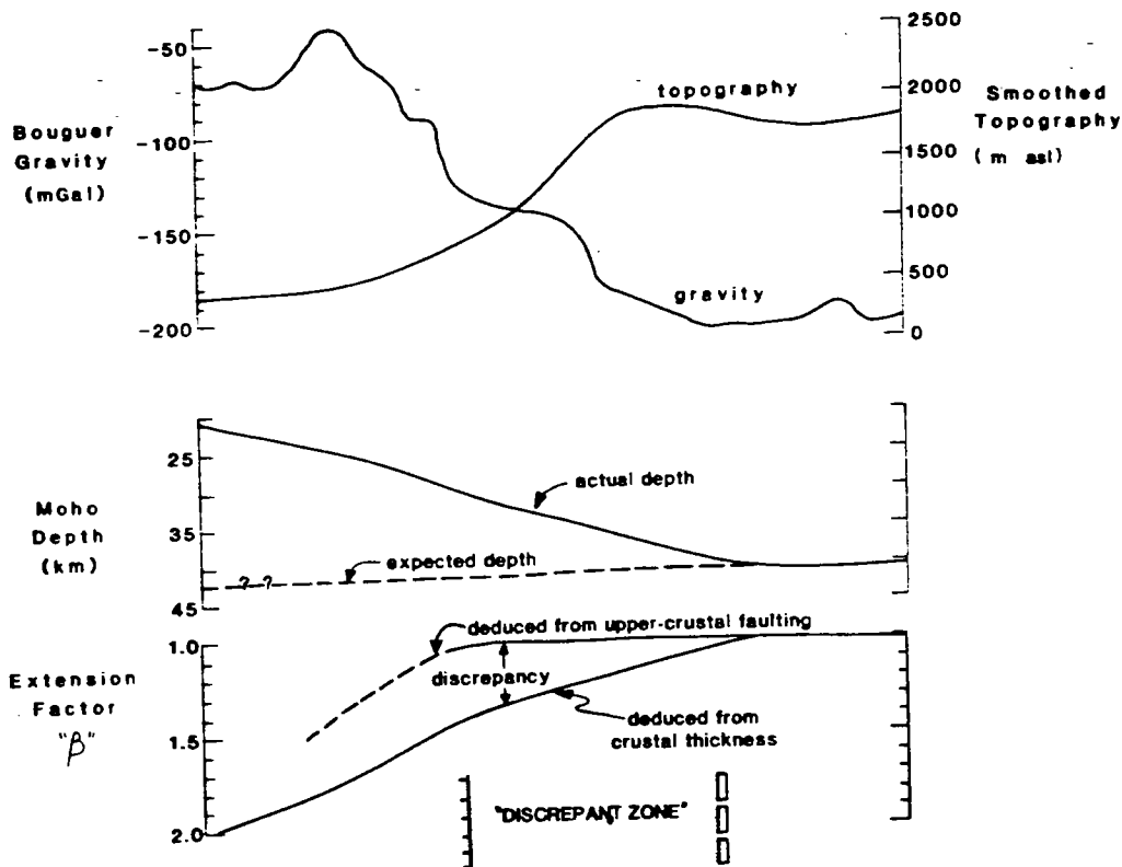
FIG. 10. Data along section line in Fig. 9 showing position of discrepant zone. Line marked "expected depth" is the probable Moho configuration before extension. Gravity and topography from Eaton et al. (1979).
