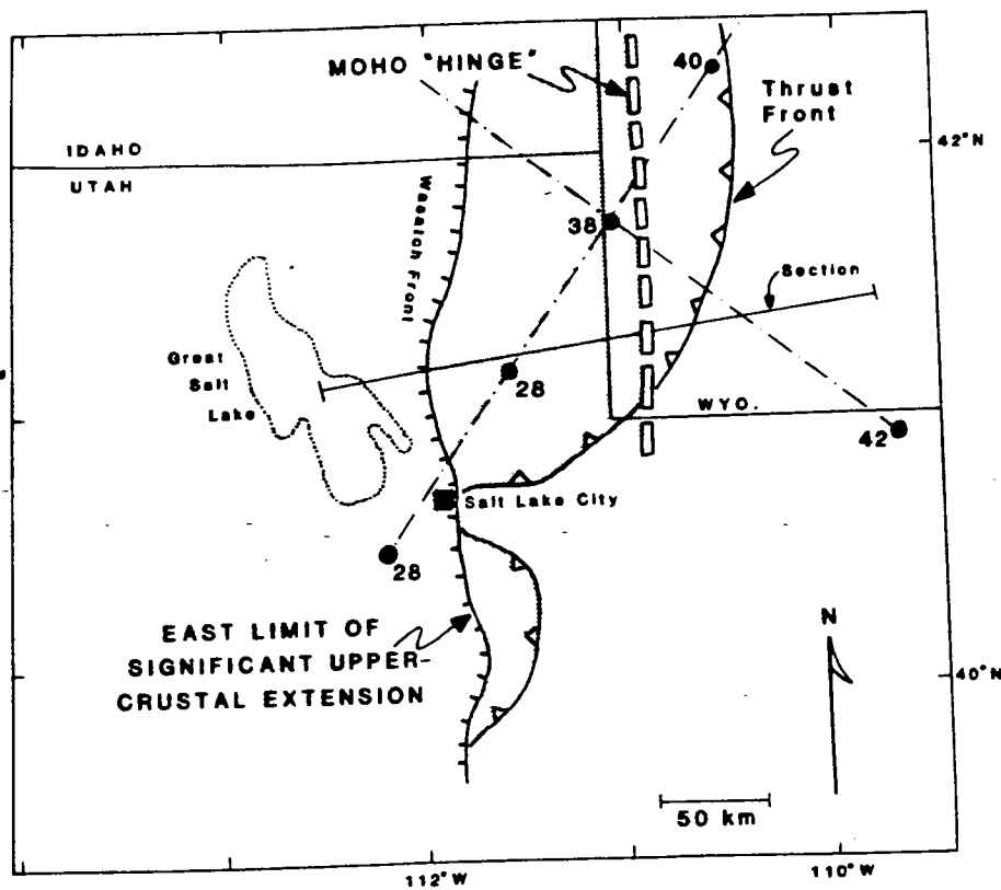
FIG. 7. Map showing positions of tectonic elements and refraction lines, which may indicate a discrepancy between crustal thickness deduced from surface faulting and that actually measured. Refraction lines and interpretations from Braile et al. (1974). Section line refers to Fig. 8.
