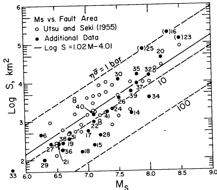
FIG. 5. Relation between M_S and S (aftershock area, fault surface area). The straight lines are for constant apparent stress. The rigidity \mu and stress drop of 3 \times 10^{11} dyne/cm 2 and 60 bars are used.
