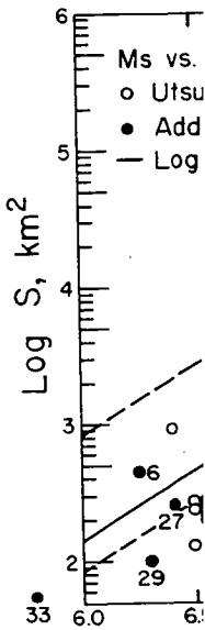
FIG. 5. Relation between M_S and constant apparent stress. The right
