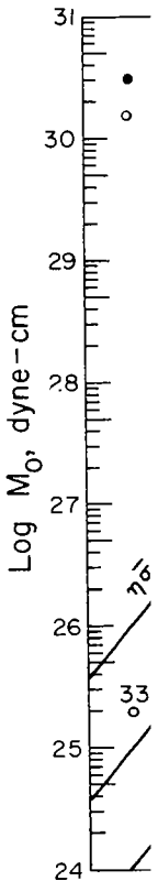
FIG. 4. Relation between M_S (20-sec surface apparent stress) and M_0 .
