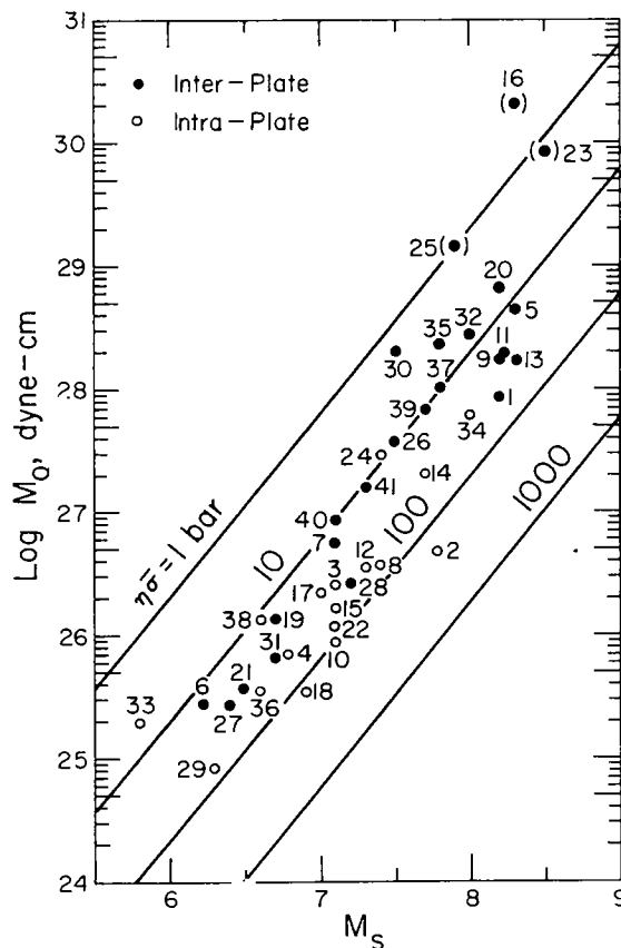
FIG. 4. Relation between M_S (20-sec surface-wave magnitude) and M_0 . The straight lines are for constant apparent stress. A rigidity of 3 \times 10^{11} dyne/cm 2 is used.
