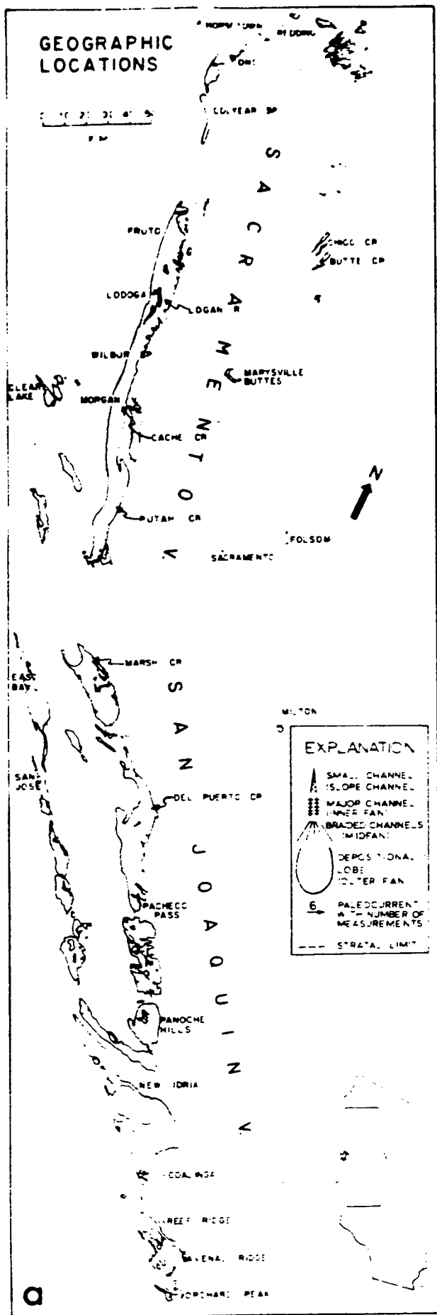
Figure 3. (a) Map showing geographic locations. Upper Cretaceous outcrops are delineated by solid lines. Stratal limits are determined by surface exposures as well as subsurface data from Bowen (1962, Pls. 5, 14, 15, 16, 17, 18.). The Great Valley consists of the Sacramento Valley in the north and the San Joaquin Valley in the south. (b) Schematic paleogeographic map for the early Cenomanian.
