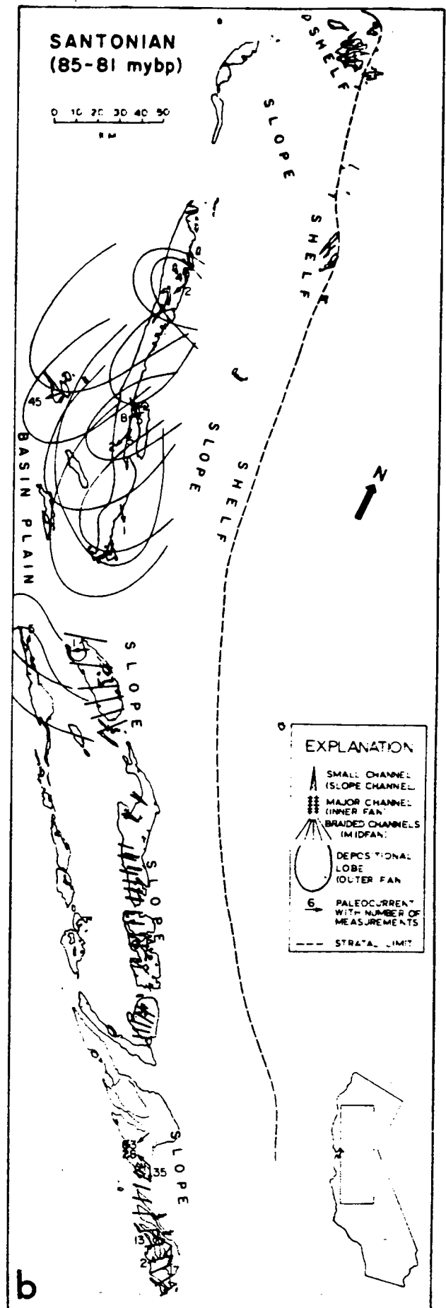
Figure 5. (a) Schematic paleogeographic map for the Coniacian. (b) Schematic paleogeographic map for the Santonian.
