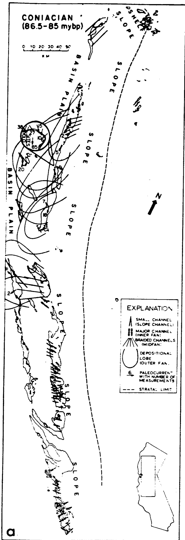
Figure 5. (a) Schematic paleogeographic map for the Coniacian. (b) Schematic paleogeographic map for the Santonian.
