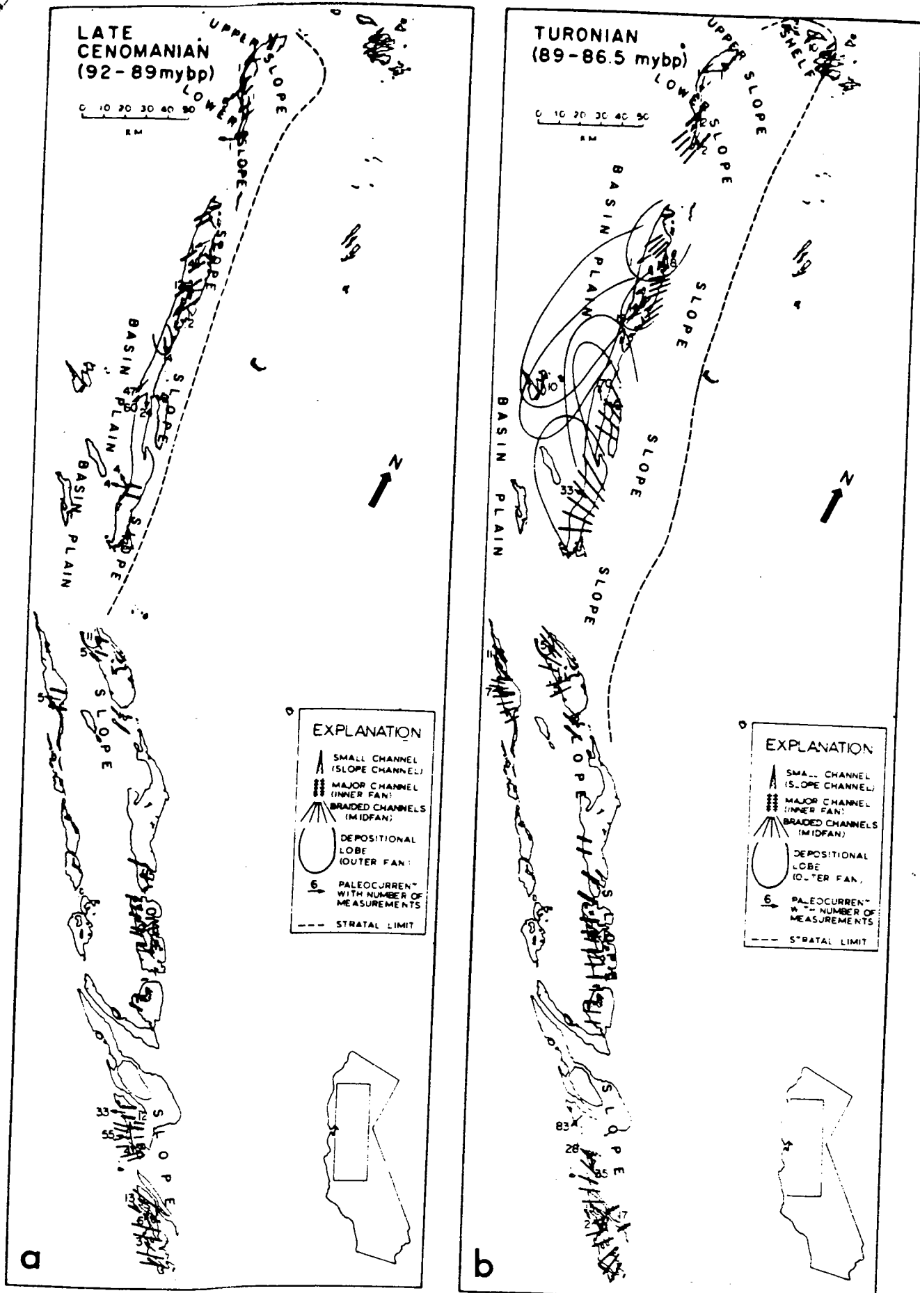
Figure 4. (a) Schematic paleogeographic map for the late Cenomanian. (b) Schematic paleogeographic map for the Turonian.
