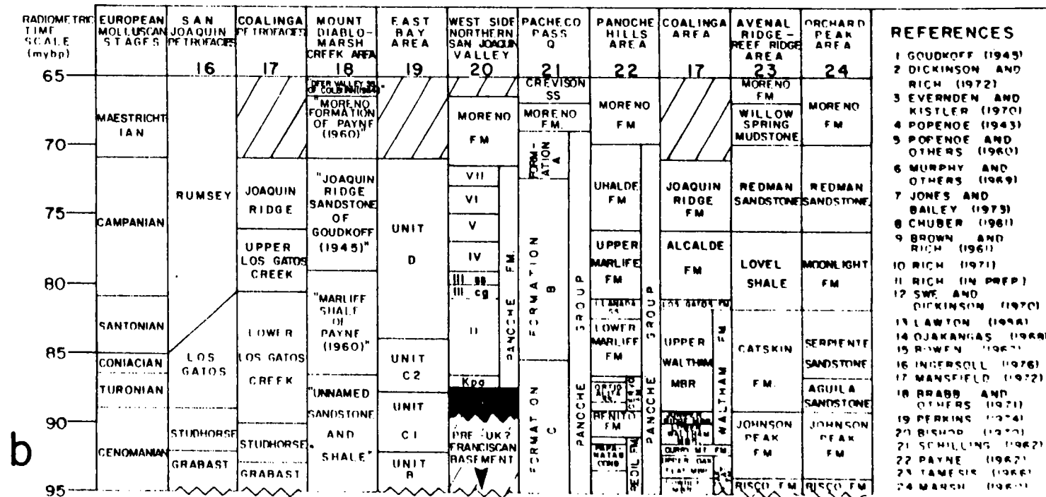
Figure 2. Correlation chart of the Upper Cretaceous part of the Great Valley Sequence and age equivalents. North is to the left for both the Sacramento Valley (a) and the San Joaquin Valley (b). Black areas indicate strata missing for tectonic reasons; slanted lines indicate strata missing due to nondeposition, erosion, or burial.
