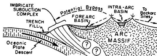
FIG. 6—Diagram showing sediment dispersal (dashed arrows) from active magmatic arc orogen, in which arc massif may be capped by undissected volcanic cover, or may include exposures of dissected plutonic and metamorphic rocks partly masked by scattered volcanic cover (see text for discussion).
