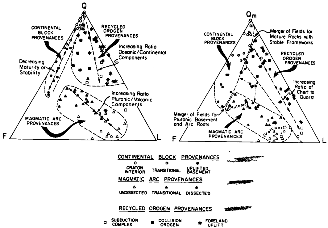
FIG. 1—Triangular QFL plot showing mean framework modes for selected sandstone suites derived from different types of provenances (data from Table 1): Q is total quartzose grains, including monocrystalline Qm and polycrystalline Qp varieties; F is total feldspar grains (all are monocrystalline); L is total unstable lithic fragments (all are polycrystalline).
