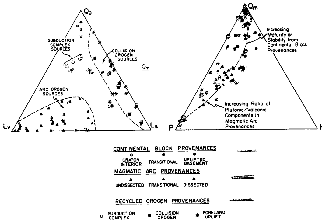
FIG. 3—Triangular Q_pL_vL_s plot showing mean proportions of polycrystalline lithic fragments for selected sandstone suites derived from different types of provenances (data from Table 1): Q_p is polycrystalline quartzose grains, mainly chert; L_v is total volcanic-metavolcanic rock fragments; L_s is unstable sedimentary-metasedimentary rock fragments.
