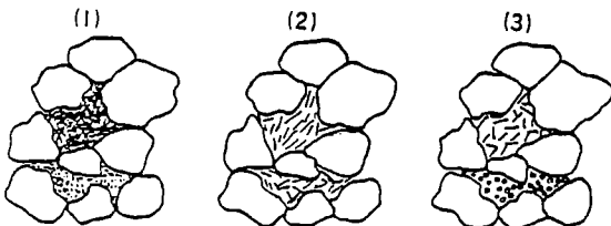
FIG. 2.—Criteria for recognition of pseudomatrix (see text): (1) criterion a, wisps extended between rigid grains, (2) criterion b, concentric form of pseudofluidal internal fabric; (3) criterion c, gaps in framework with relict lithic fragment textures.
