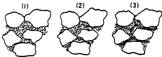
FIG. 1.—Criteria for recognition of phyllosilicate cement (see text; criteria a, clear transparency, and b, monomineralogy, not shown): (1) criterion c, radial crystal platelets; (2) criterion d, concentric color zonation; (3) criteria e, medial sutures.
