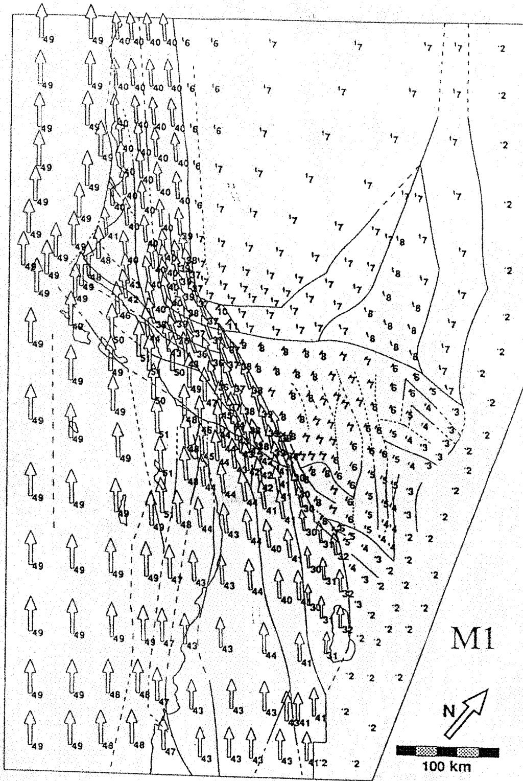
Fig. 5. Mean velocity estimates in mm/yr relative to North America for the geologically-based solution M1. The relative motion between the eastern and western boundaries is given by the NUVEL-1 Pacific relative motion minus 2 mm/yr for NUVEL-1-parallel motion east of California (see text).
