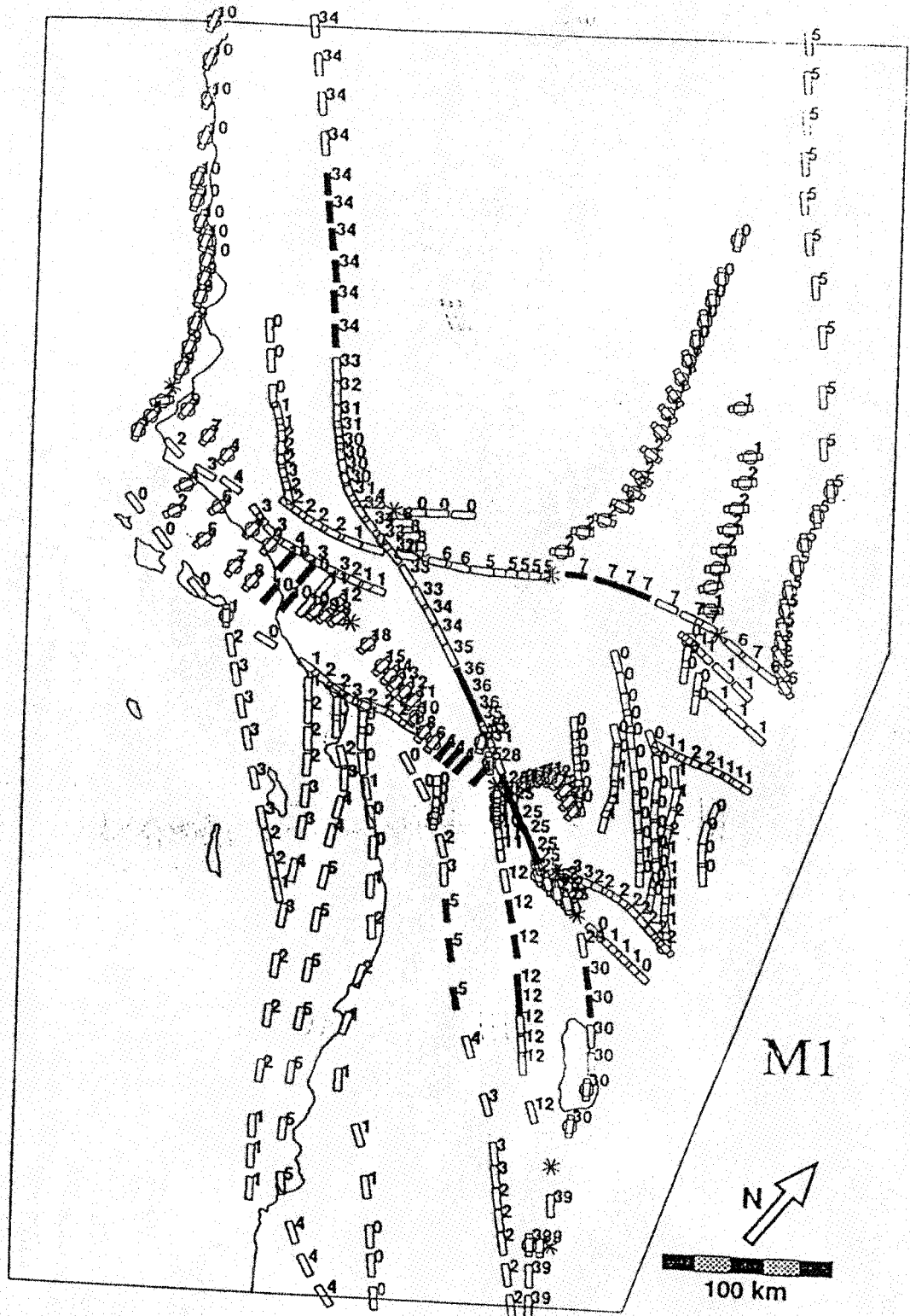
Fig. 6. Fault slip rates for the geologically-based solution M1 in mm/yr. Dark rectangles represent the mean rate data, open rectangles represent prescribed orientations; rectangles superimposed on circles represent completely unconstrained faults, stars represent triple junctions that are also unconstrained.
